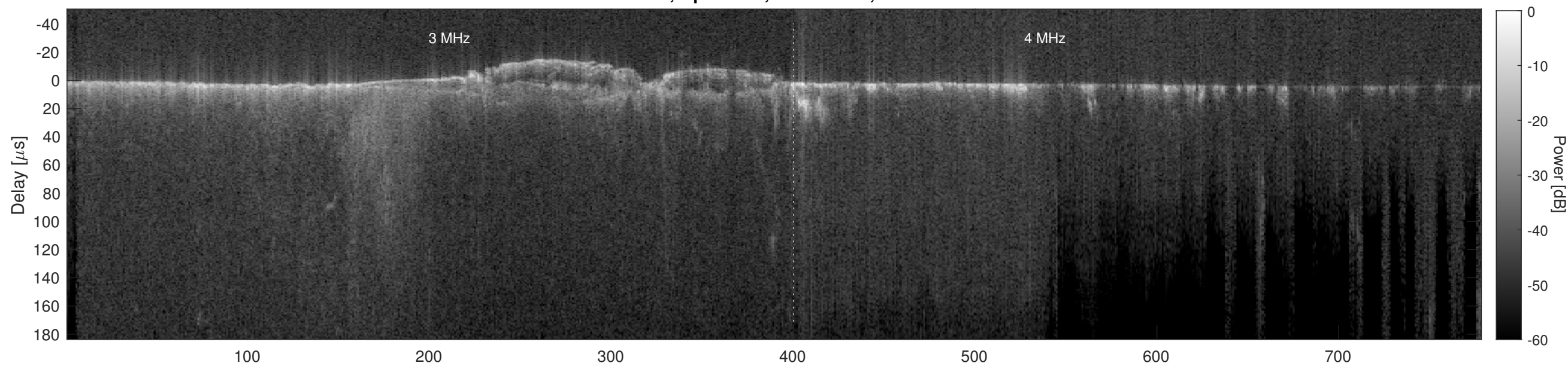
Orbit 9639, Cluttergram
