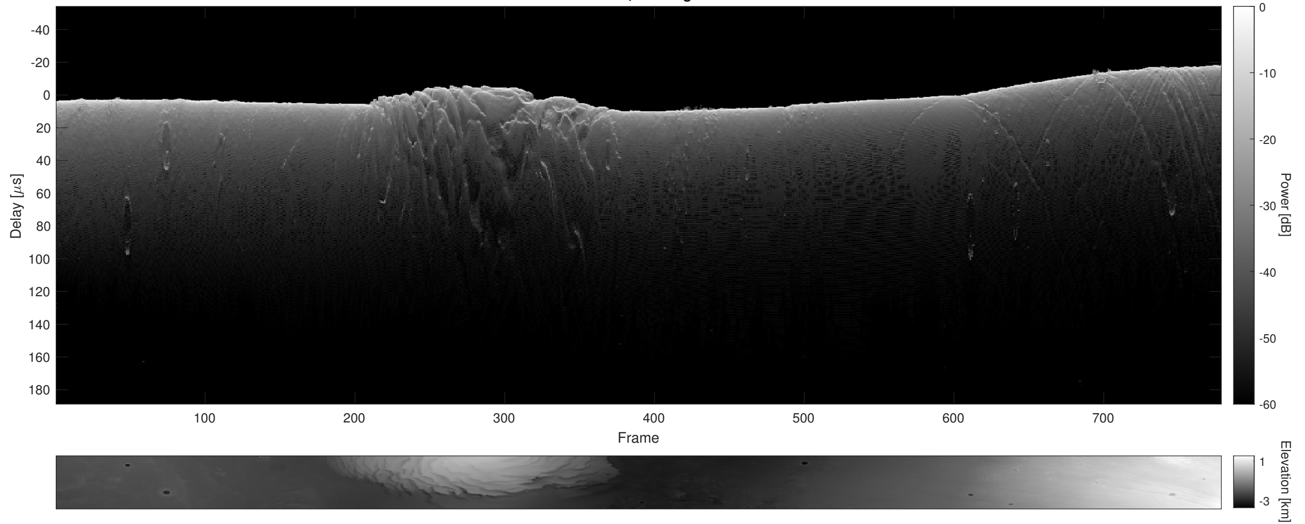
Orbit 9640, Cluttergram
