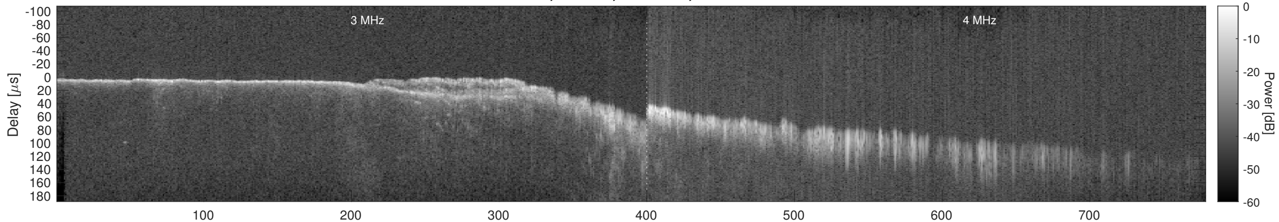
Orbit 9640, Window, Channel 2, Chapman
