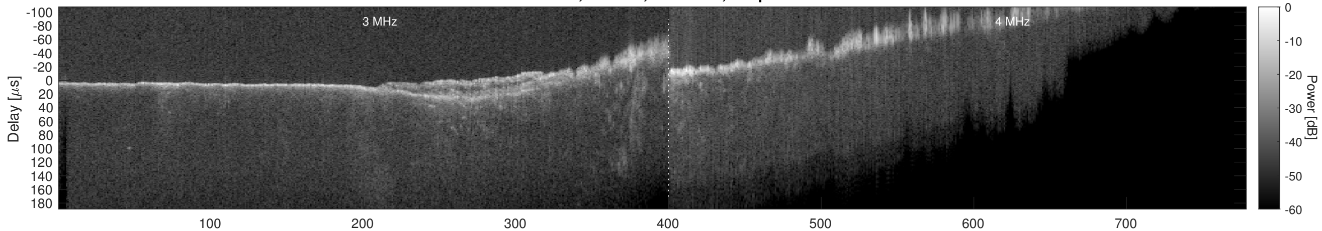
Orbit 9640, Window, Channel 2, Optimized
