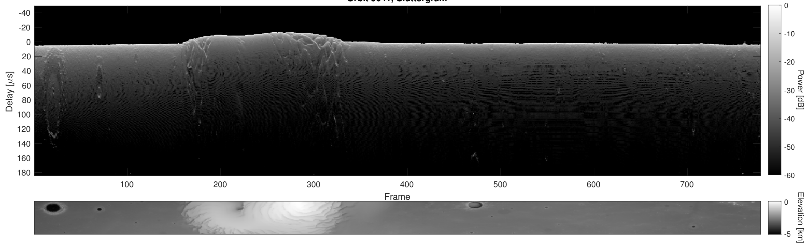
Orbit 9641, Cluttergram
