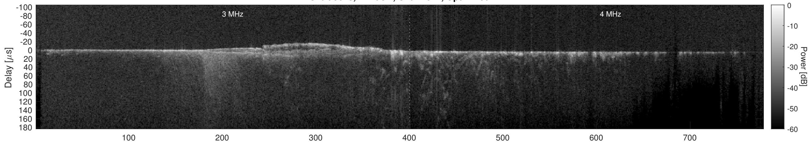
Orbit 9643, Cluttergram
