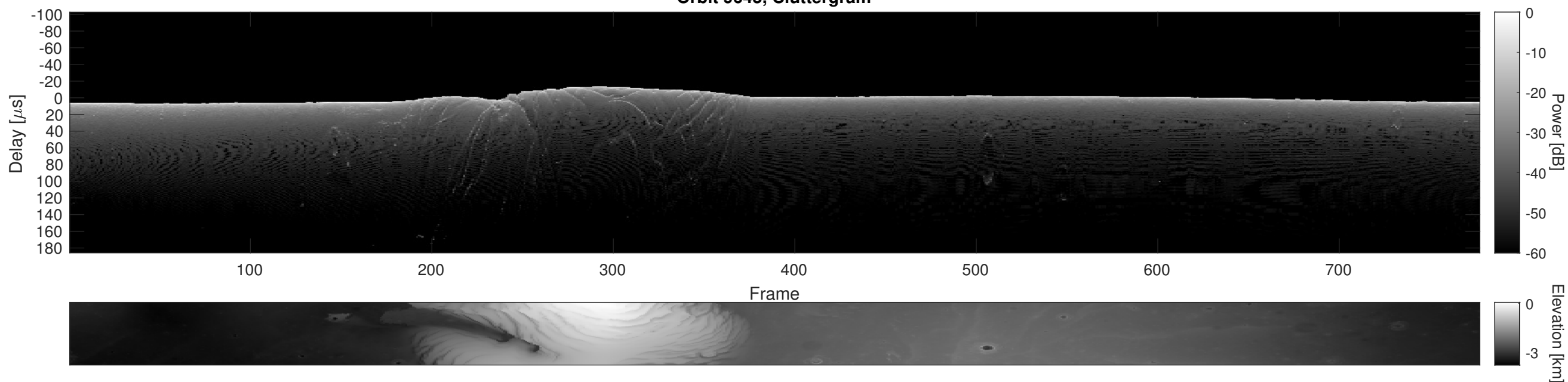
Orbit 9645, Cluttergram
