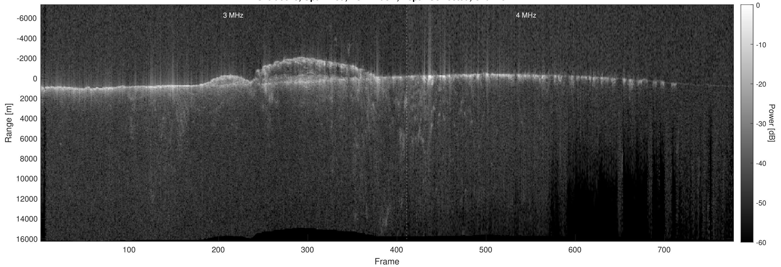
Orbit 9645, Optimized, No Window, Depth-Corrected, Channel 2
