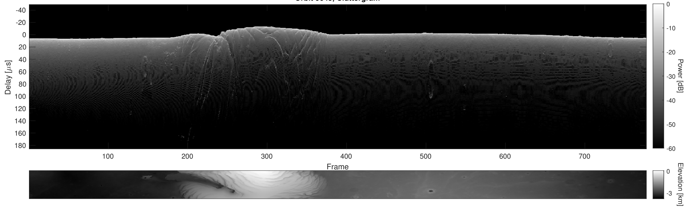
Orbit 9645, Cluttergram
