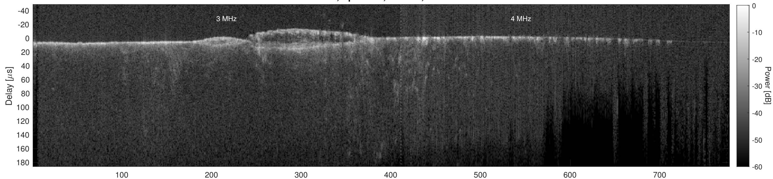
Orbit 9645, Cluttergram
