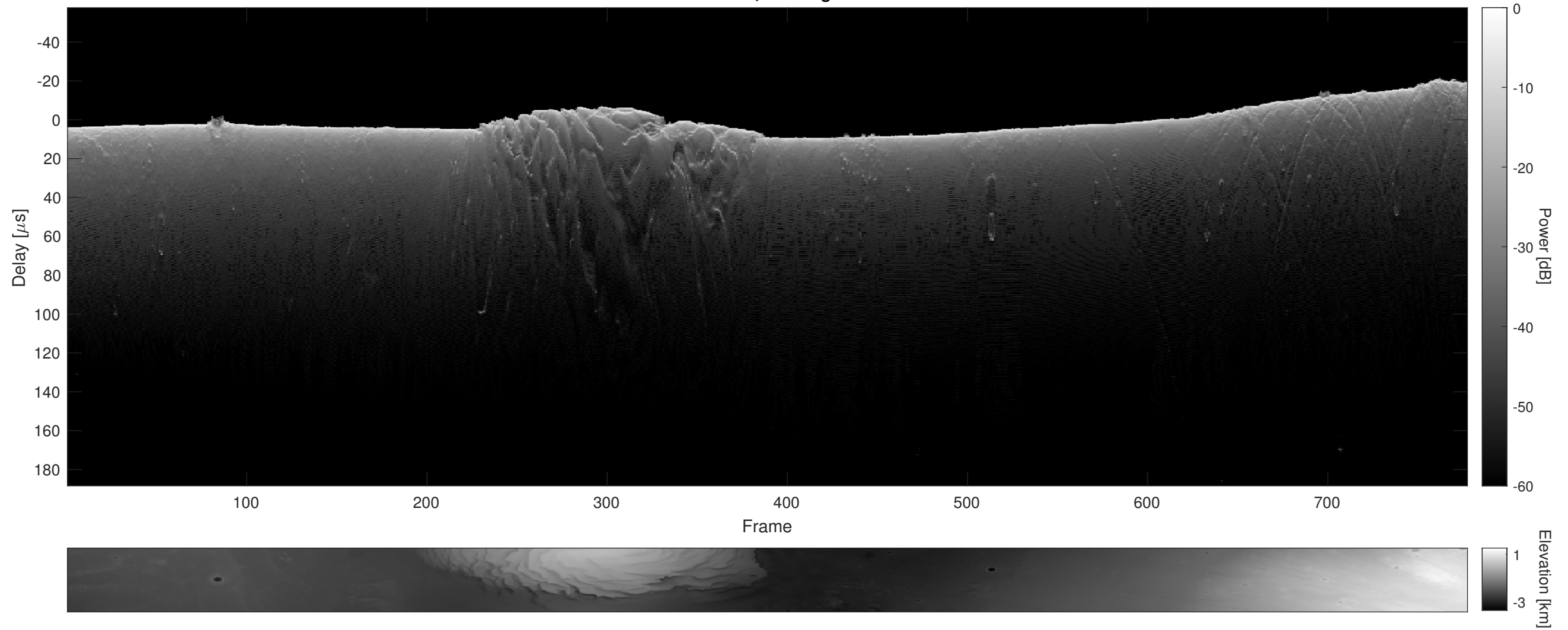
Orbit 9647, Cluttergram
