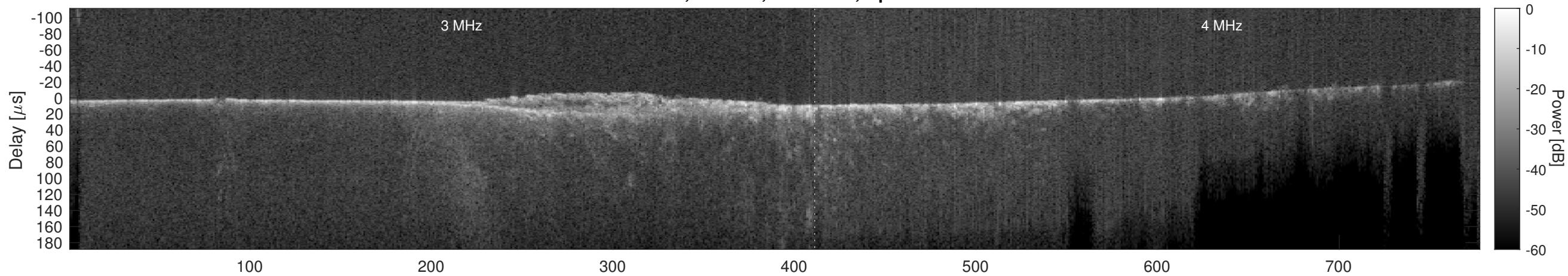
Orbit 9647, Cluttergram
