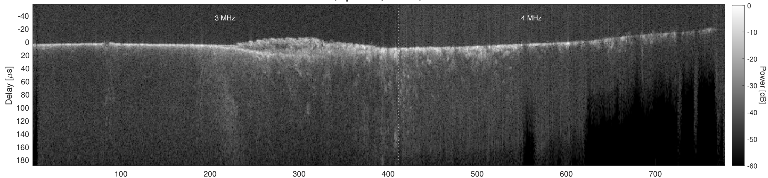
Orbit 9647, Cluttergram
