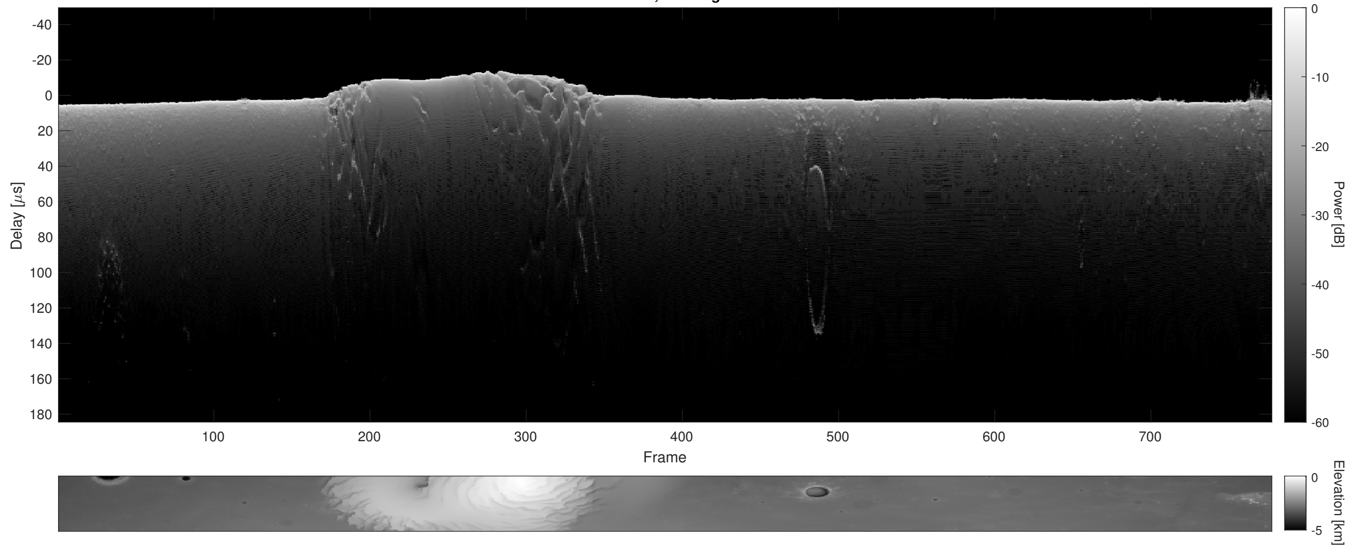
Orbit 9648, Cluttergram
