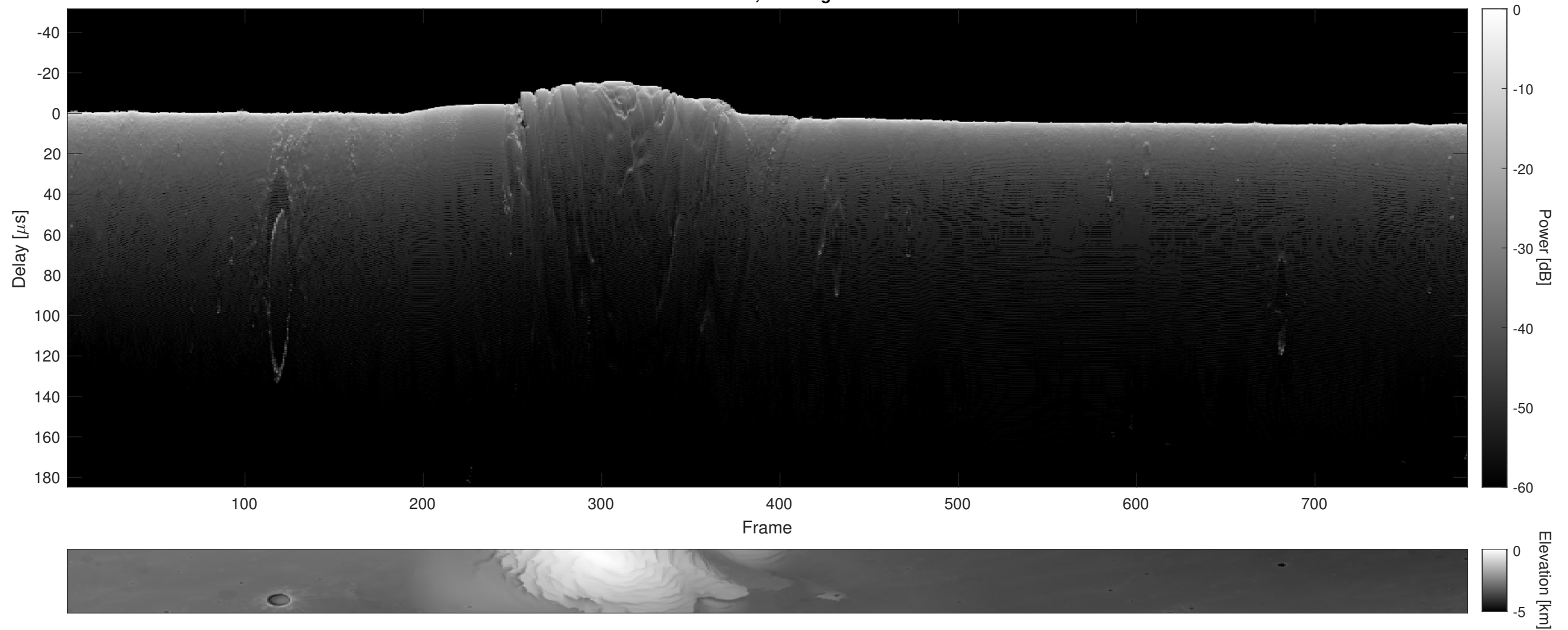
Orbit 9650, Cluttergram
