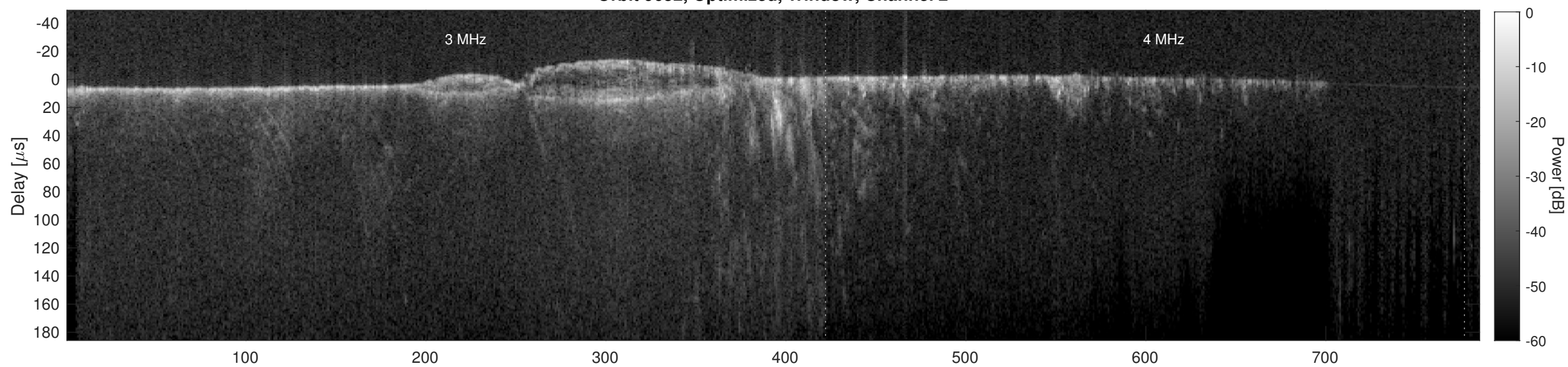
Orbit 9652, Cluttergram
