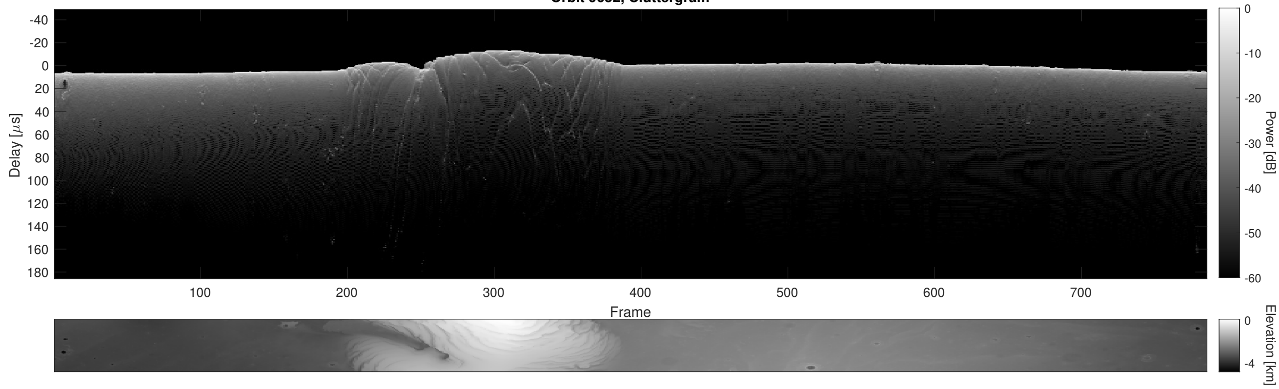
Orbit 9652, Cluttergram
