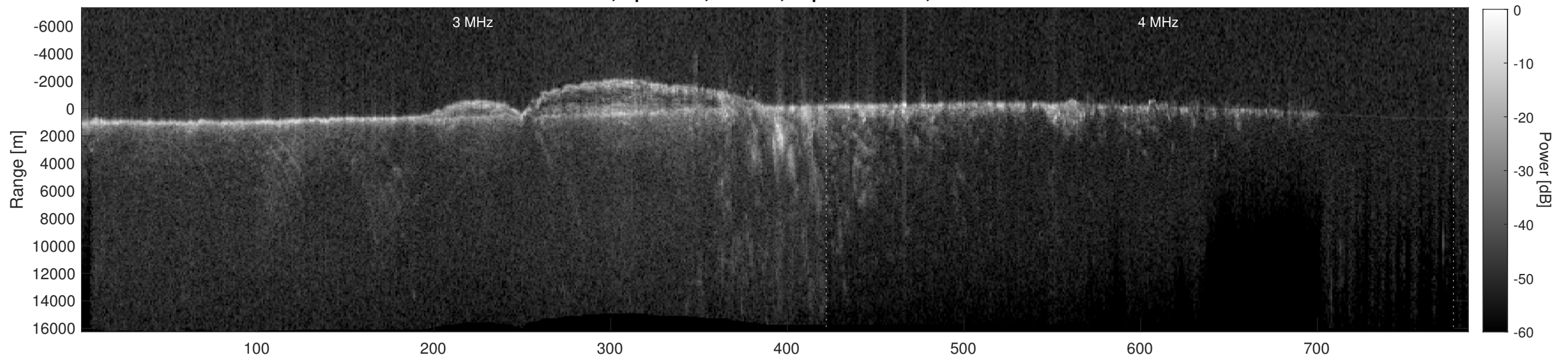
Orbit 9652, Depth-Corrected Cluttergram
