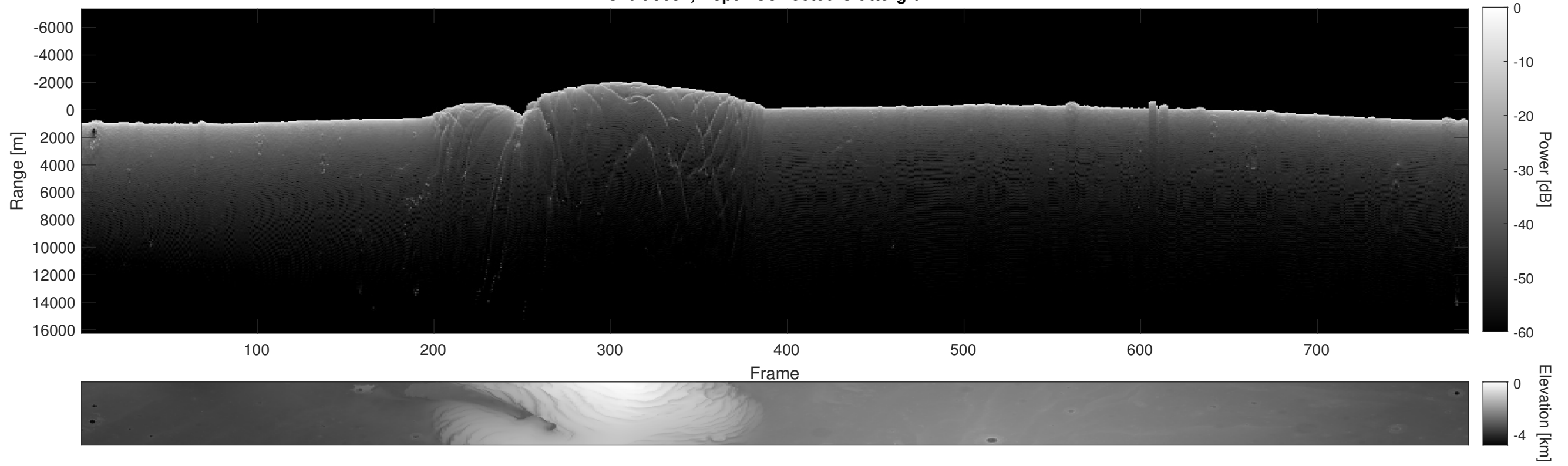
Orbit 9652, Depth-Corrected Cluttergram
