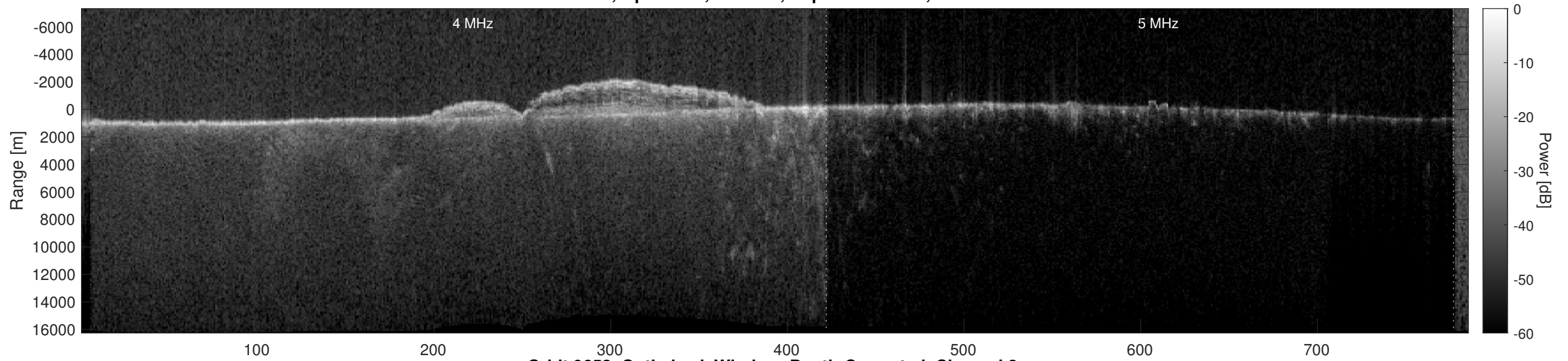
Orbit 9652, Optimized, Window, Depth-Corrected, Channel 2
