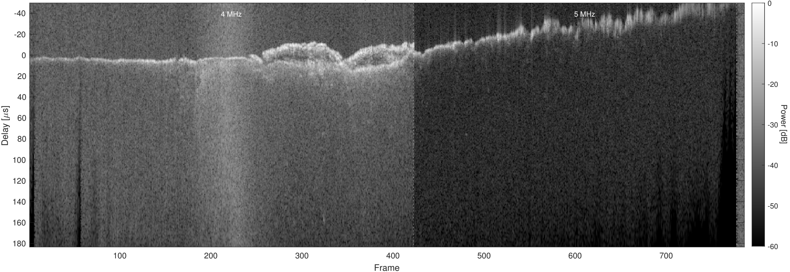
Orbit 9653, Chapman, Window, Channel 2
