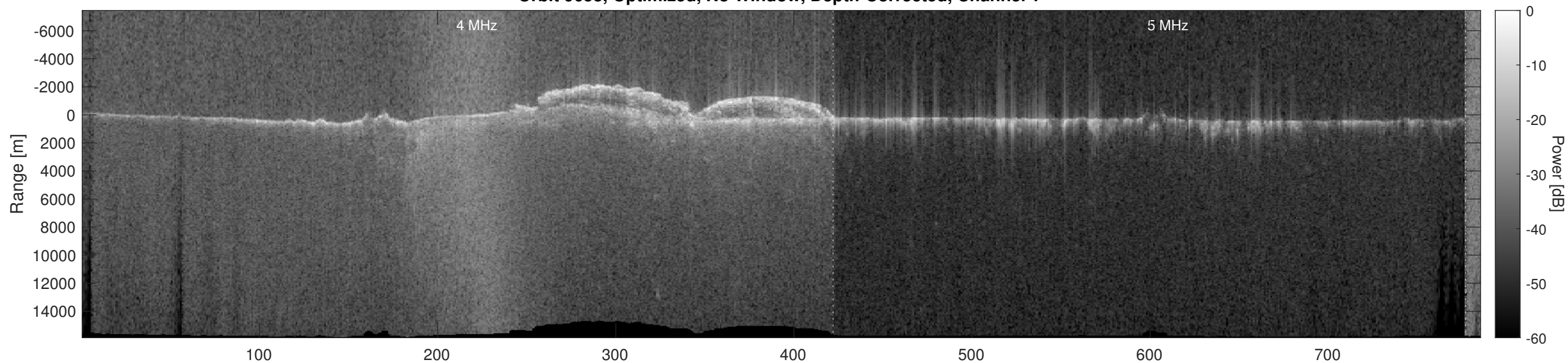
Orbit 9653, Optimized, No Window, Depth-Corrected, Channel 2
