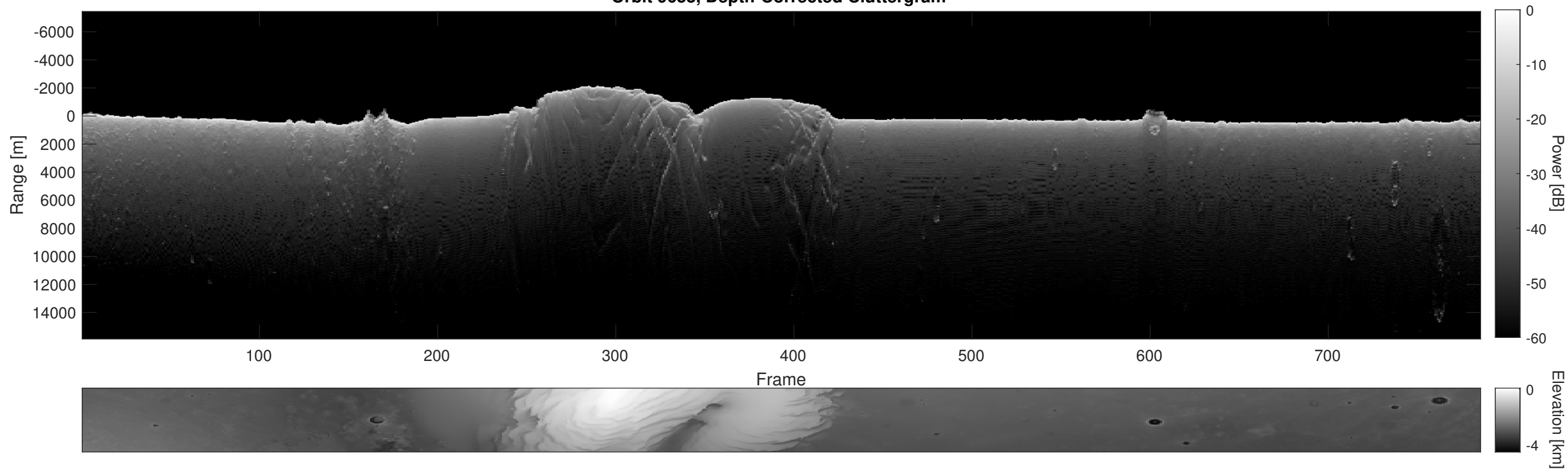
Orbit 9653, Depth-Corrected Cluttergram
