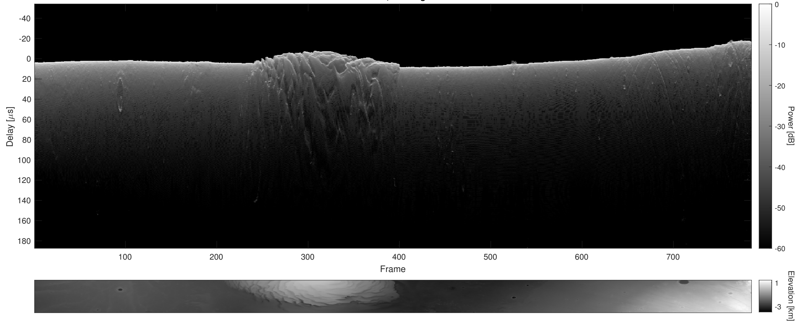
Orbit 9654, Cluttergram
