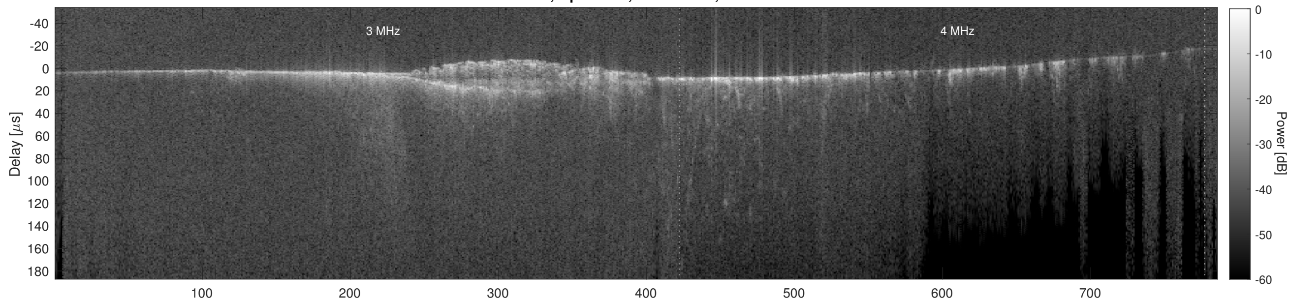
Orbit 9654, Cluttergram
