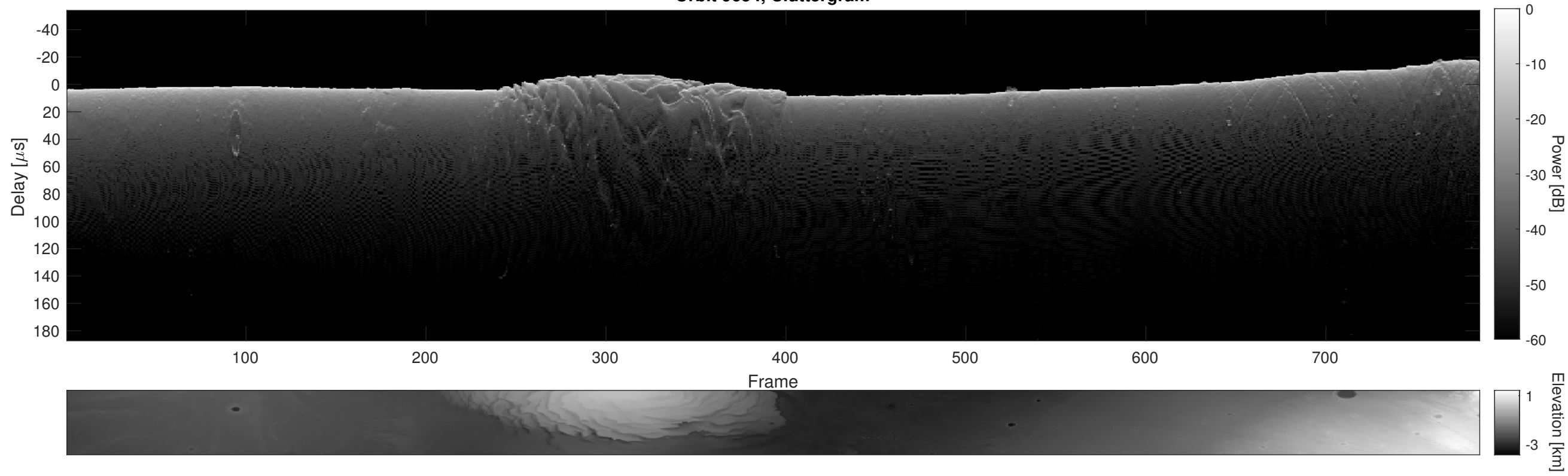
Orbit 9654, Cluttergram
