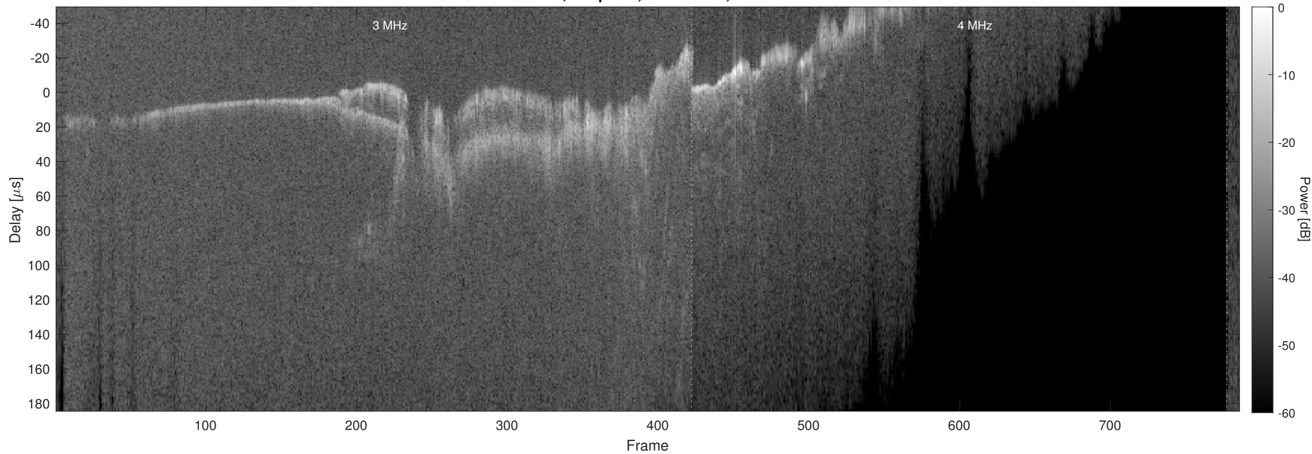
Orbit 9655, Chapman, No Window, Channel 2
