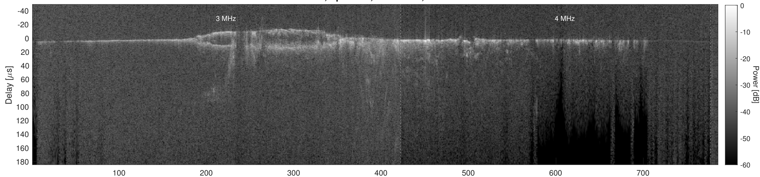
Orbit 9655, Cluttergram
