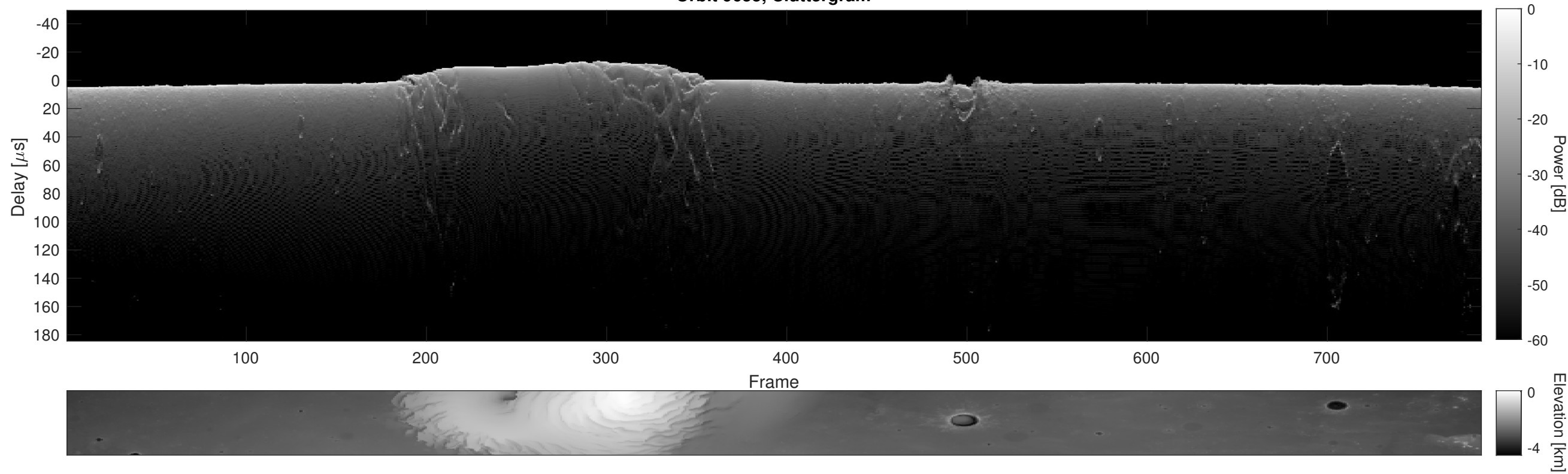
Orbit 9655, Cluttergram
