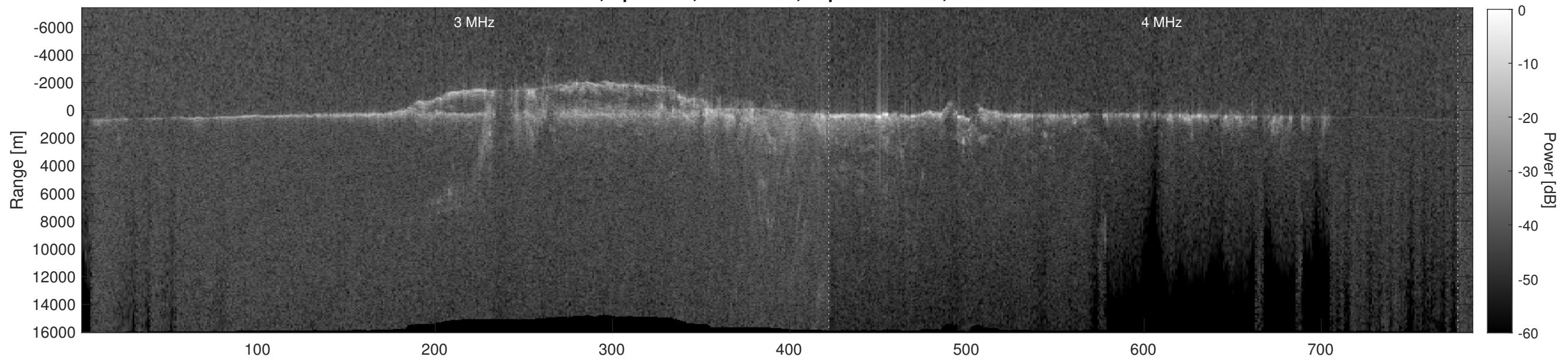
Orbit 9655, Depth-Corrected Cluttergram
