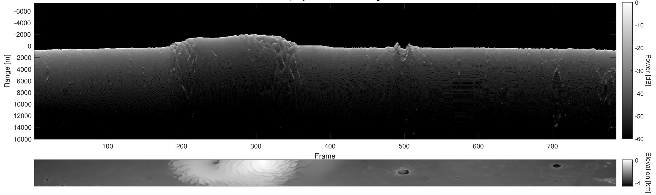
Orbit 9655, Depth-Corrected Cluttergram
