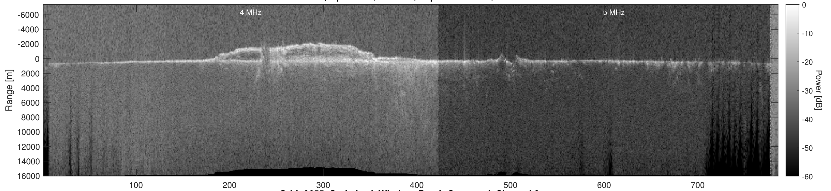
Orbit 9655, Optimized, Window, Depth-Corrected, Channel 2
