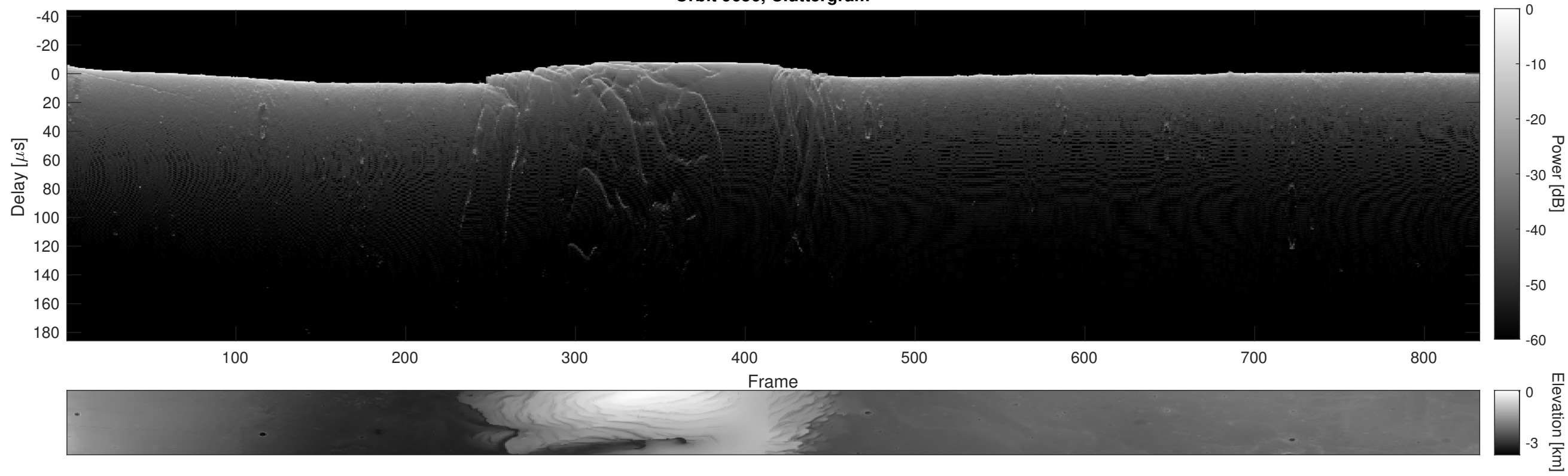
Orbit 9656, Cluttergram
