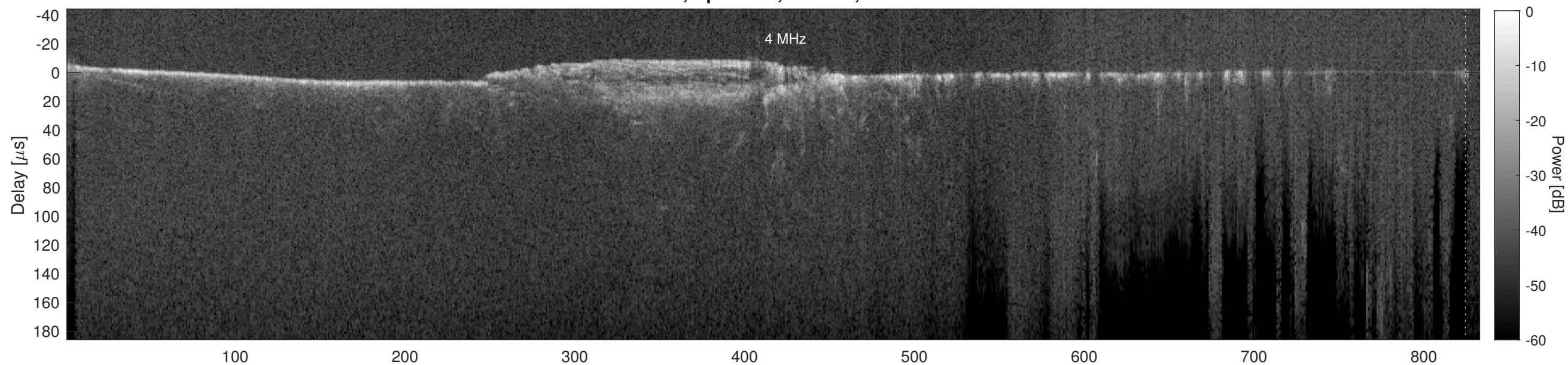
Orbit 9656, Cluttergram
