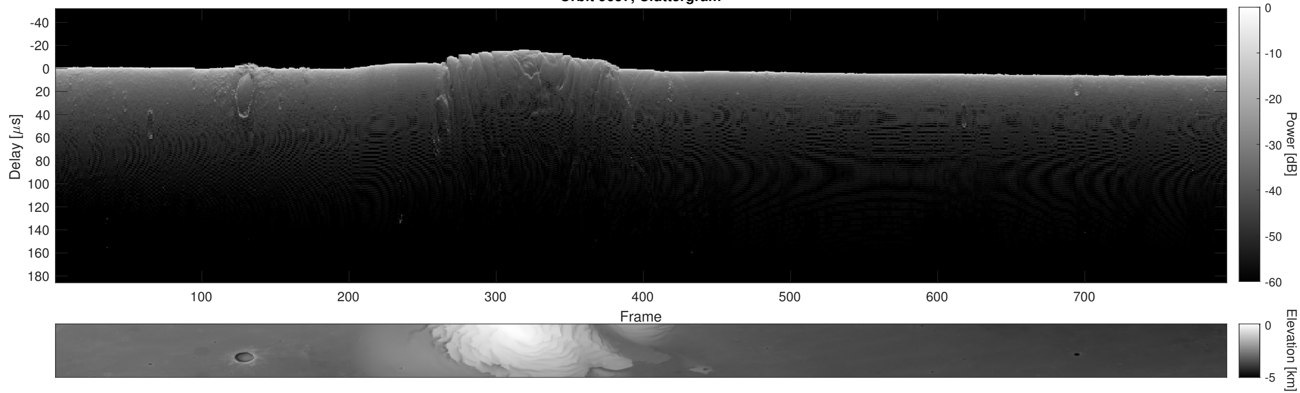
Orbit 9657, Cluttergram
