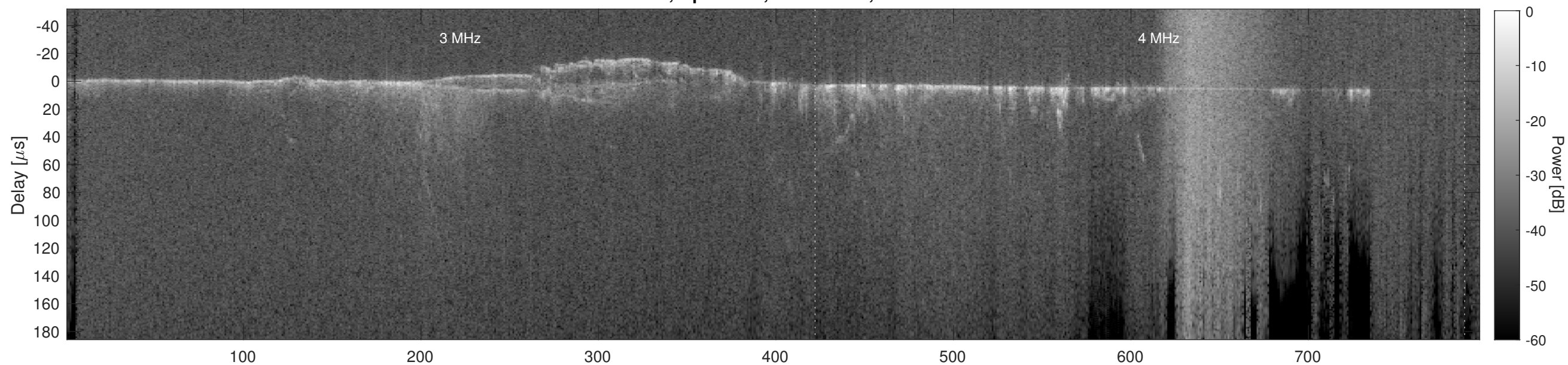
Orbit 9657, Cluttergram
