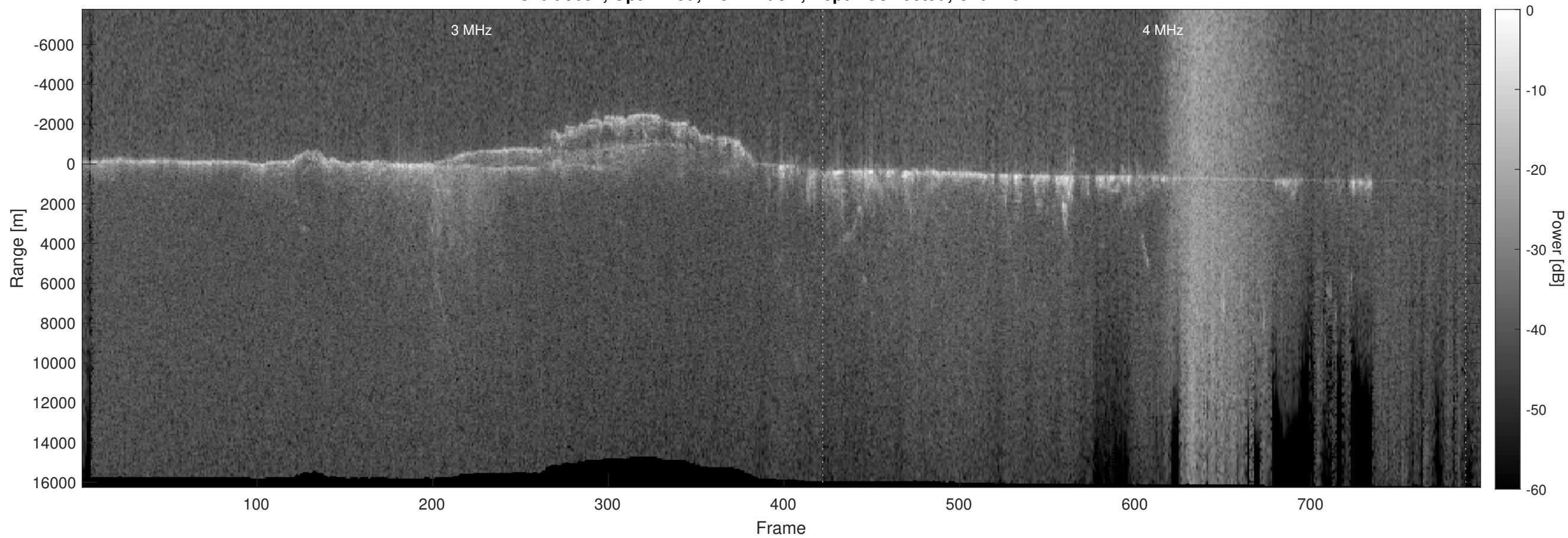
Orbit 9657, Optimized, No Window, Depth-Corrected, Channel 2
