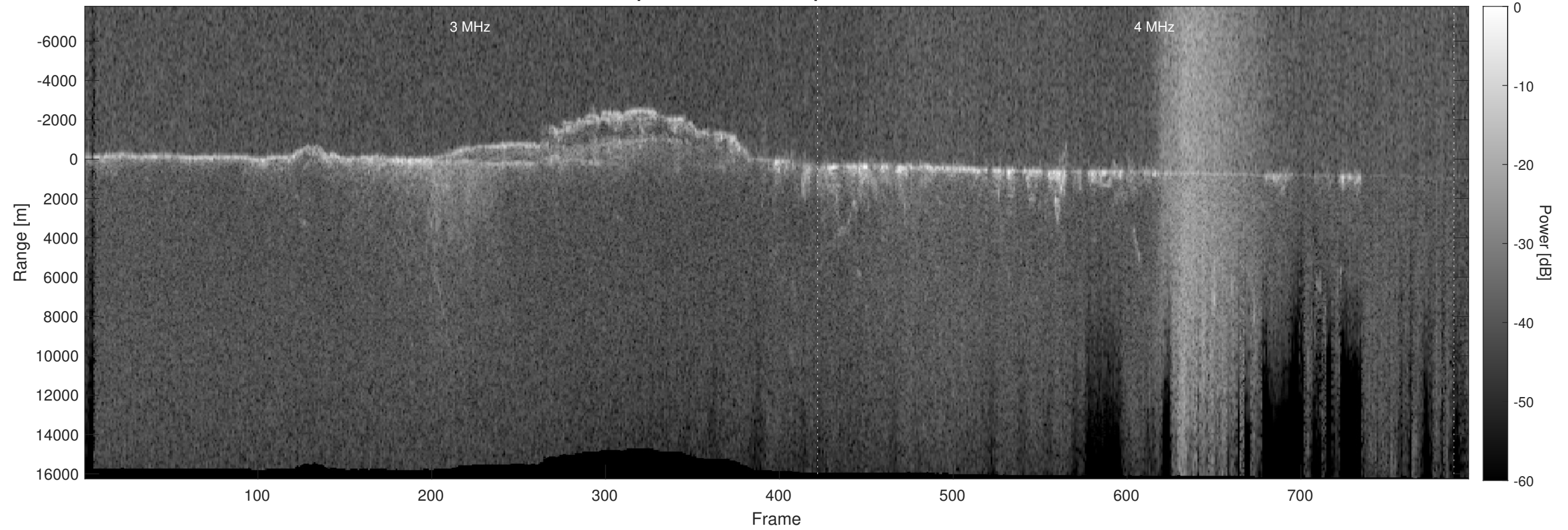
Orbit 9657, Optimized, Window, Depth-Corrected, Channel 2
