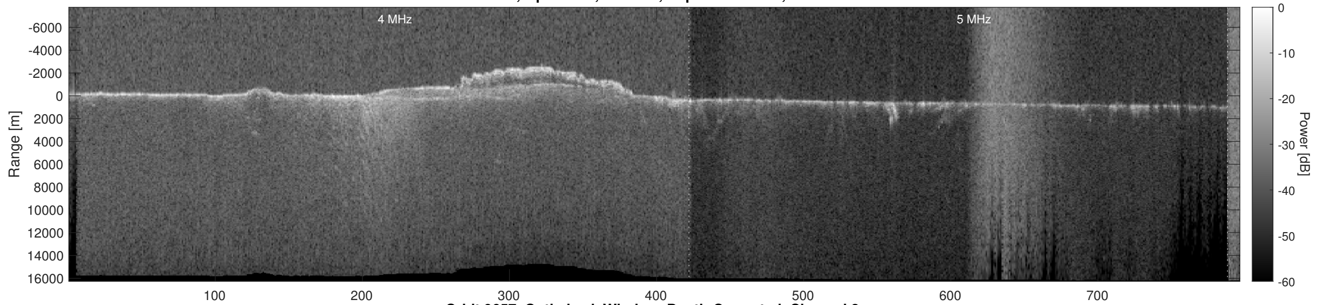
Orbit 9657, Optimized, Window, Depth-Corrected, Channel 2
