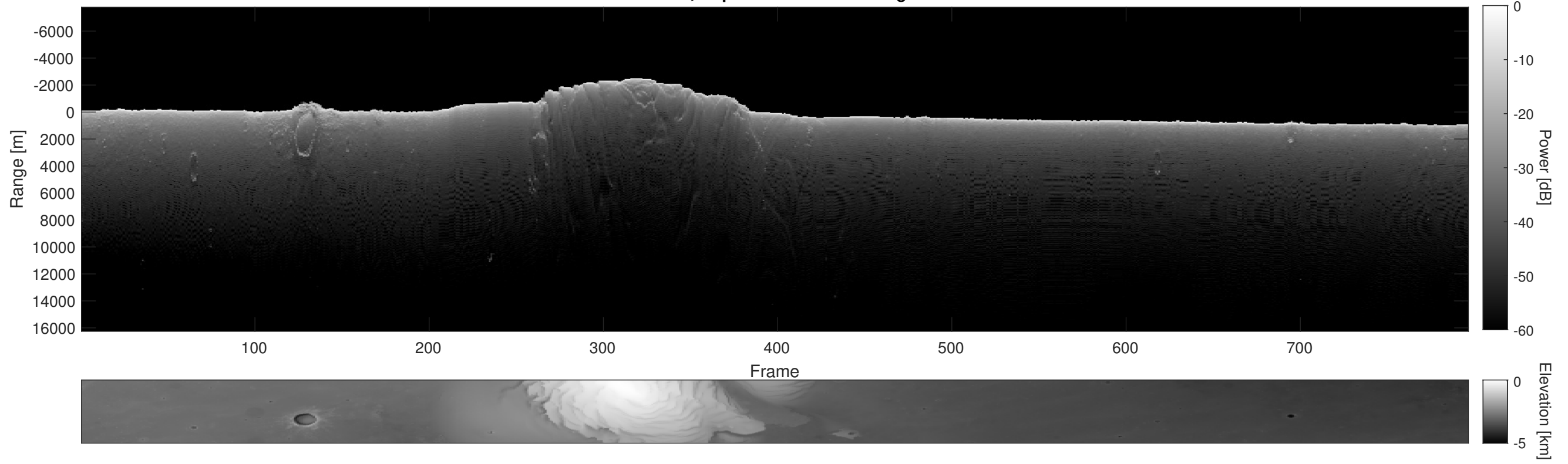
Orbit 9657, Depth-Corrected Cluttergram
