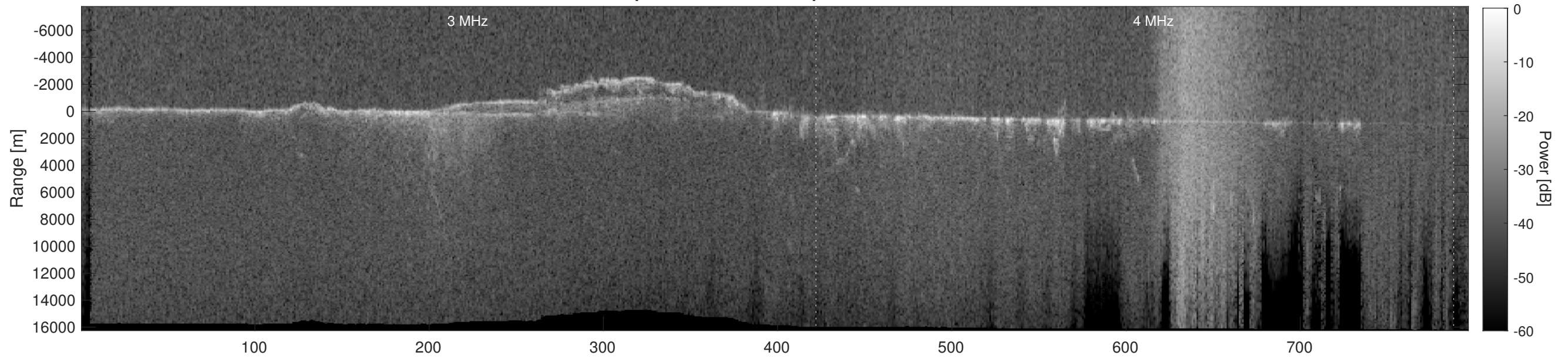
Orbit 9657, Depth-Corrected Cluttergram
