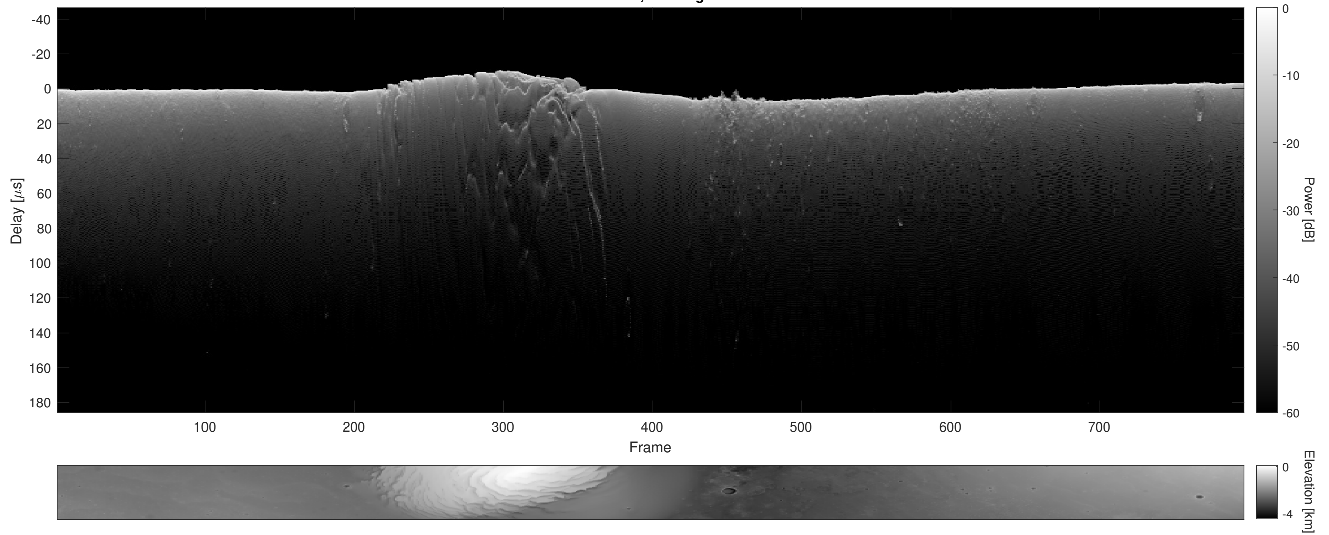
Orbit 9658, Cluttergram
