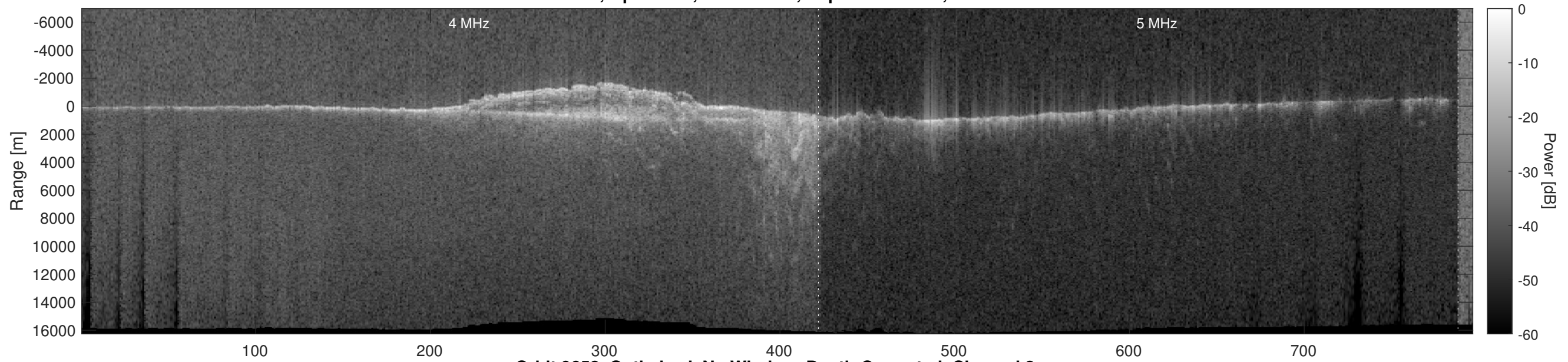
Orbit 9658, Optimized, No Window, Depth-Corrected, Channel 2
