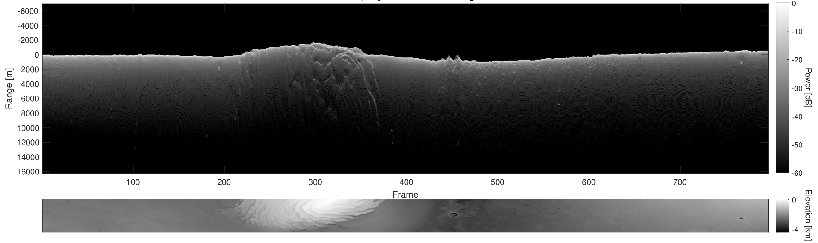
Orbit 9658, Depth-Corrected Cluttergram
