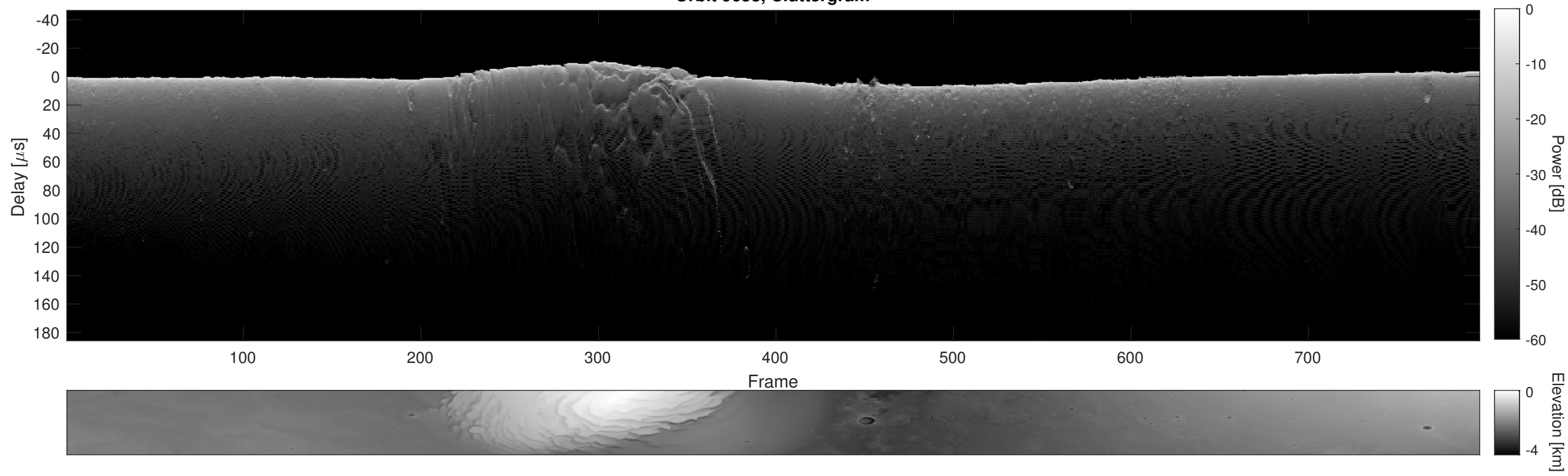
Orbit 9658, Cluttergram
