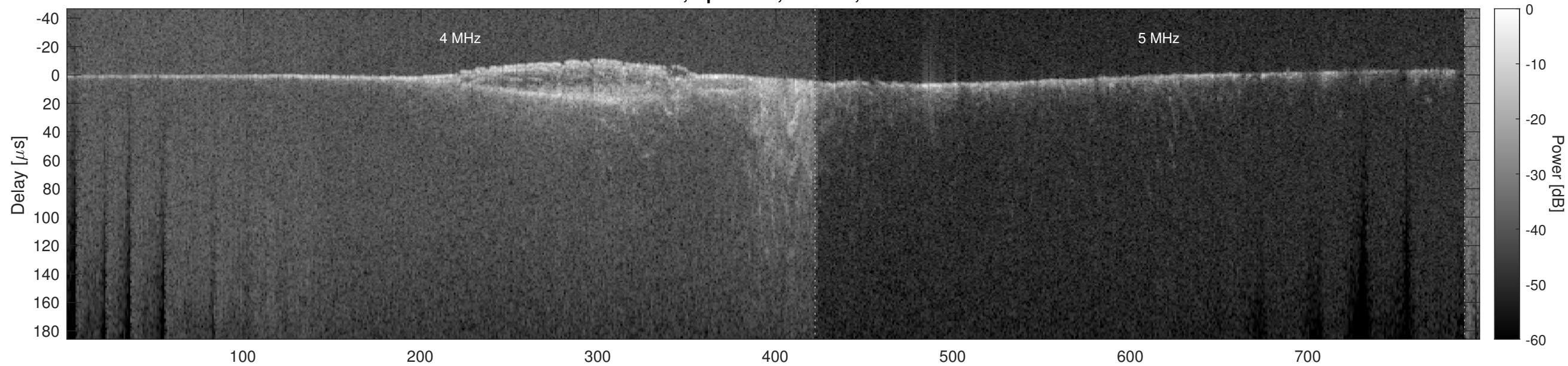
Orbit 9658, Optimized, Window, Channel 2
