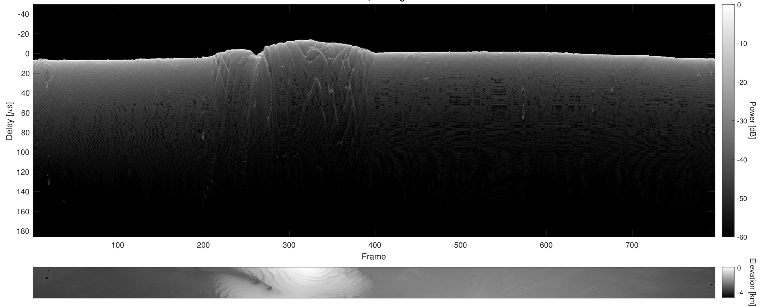
Orbit 9659, Cluttergram
