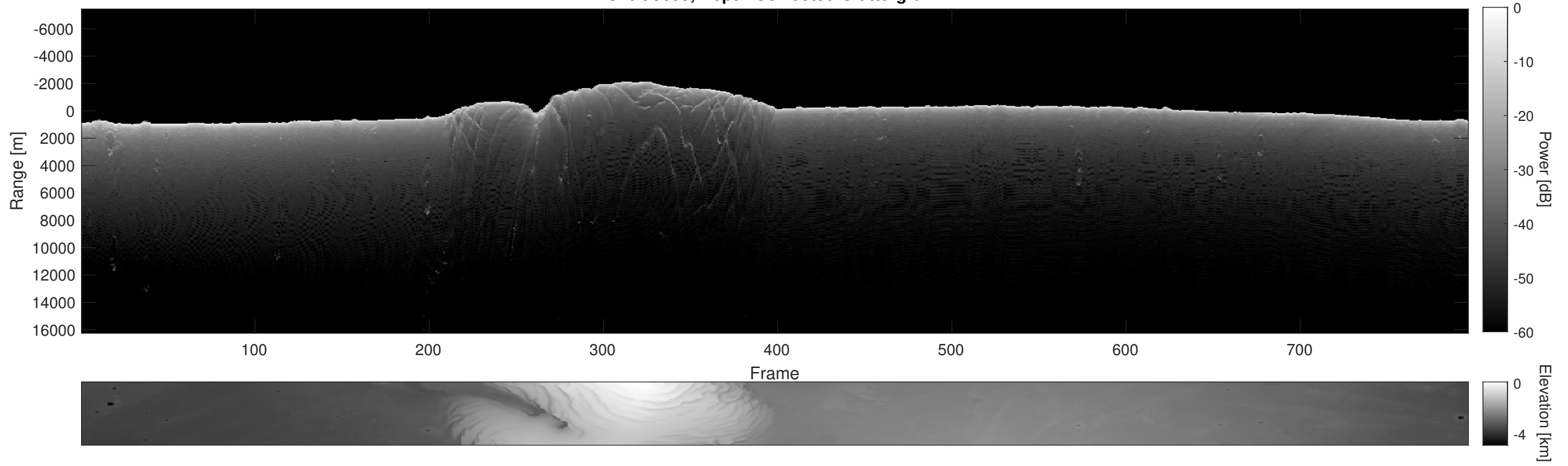
Orbit 9659, Depth-Corrected Cluttergram
