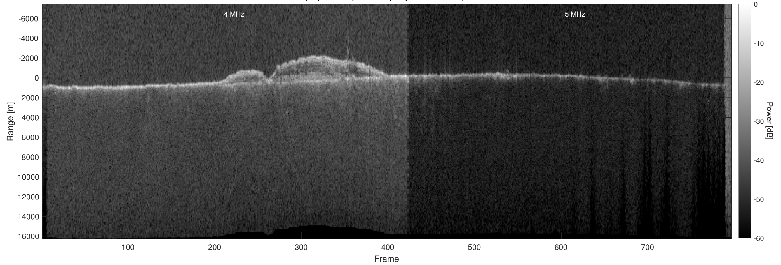
Orbit 9659, Optimized, Window, Depth-Corrected, Channel 2
