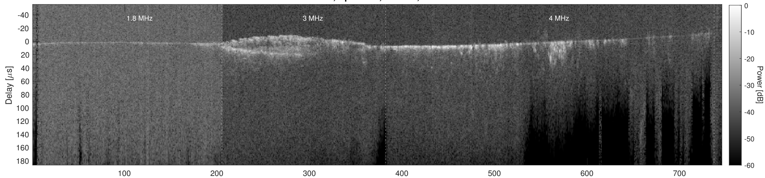
Orbit 9661, Cluttergram
