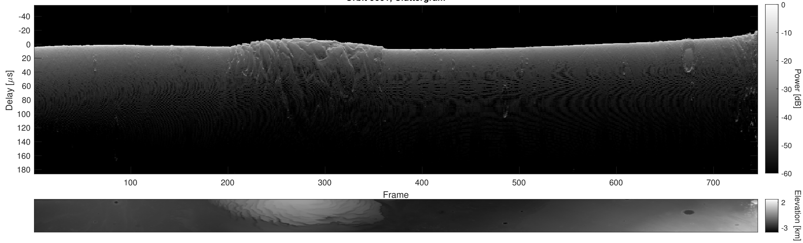
Orbit 9661, Cluttergram
