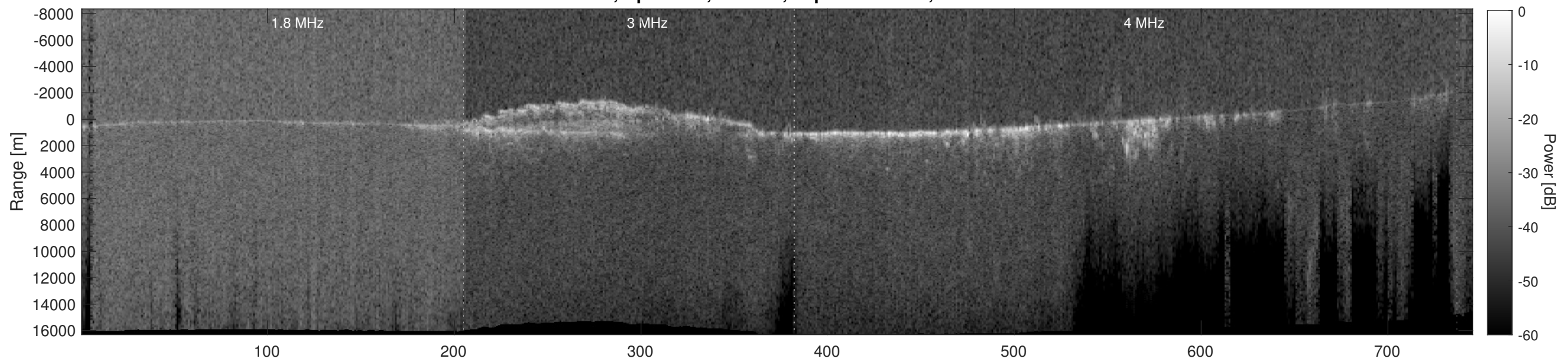
Orbit 9661, Depth-Corrected Cluttergram
