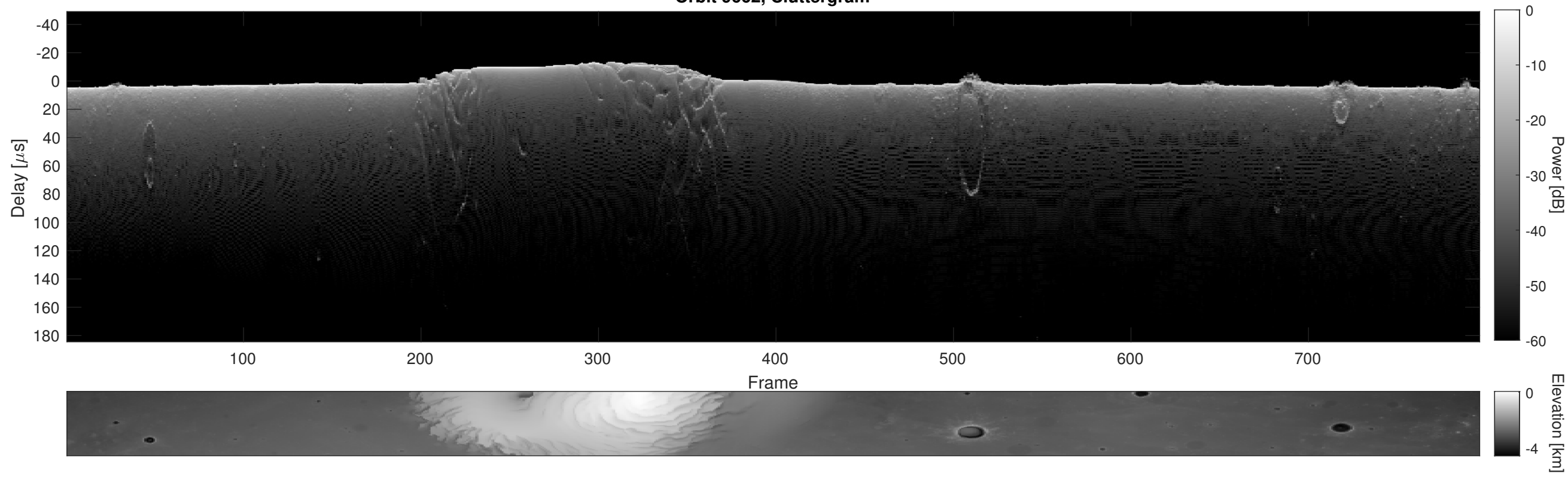
Orbit 9662, Cluttergram
