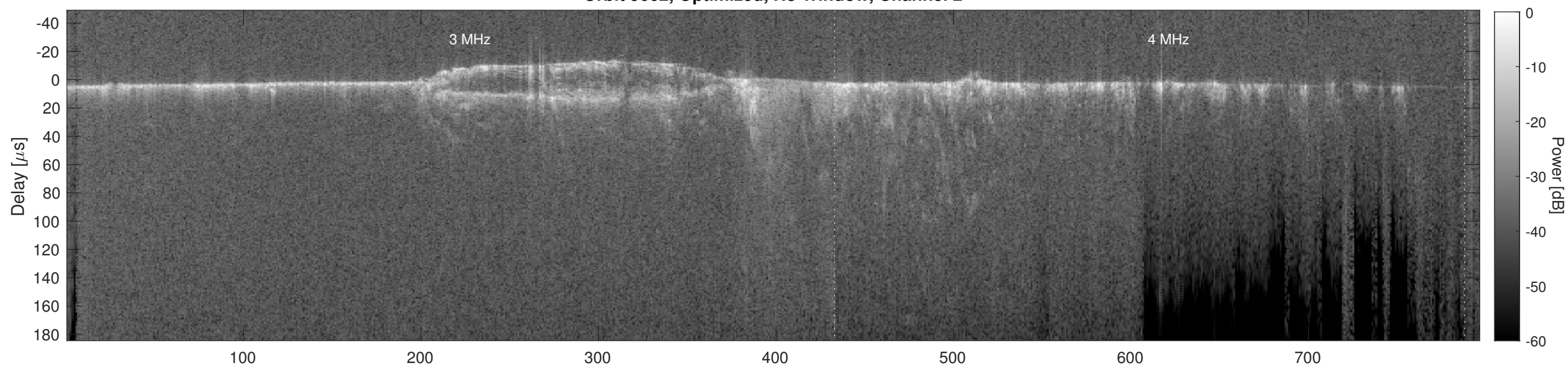
Orbit 9662, Cluttergram
