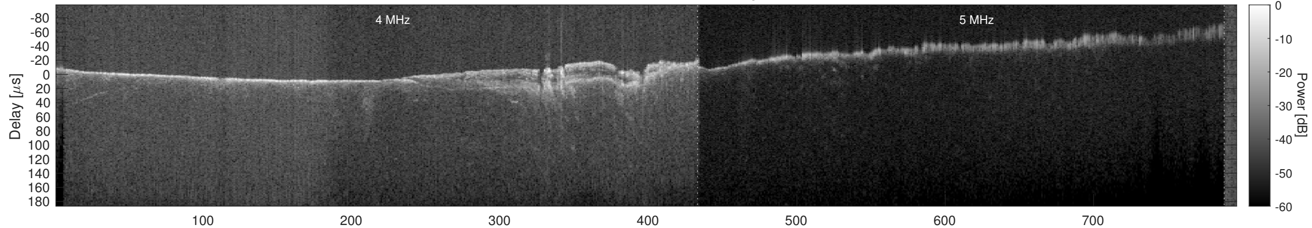
Orbit 9663, Window, Channel 1, Optimized
