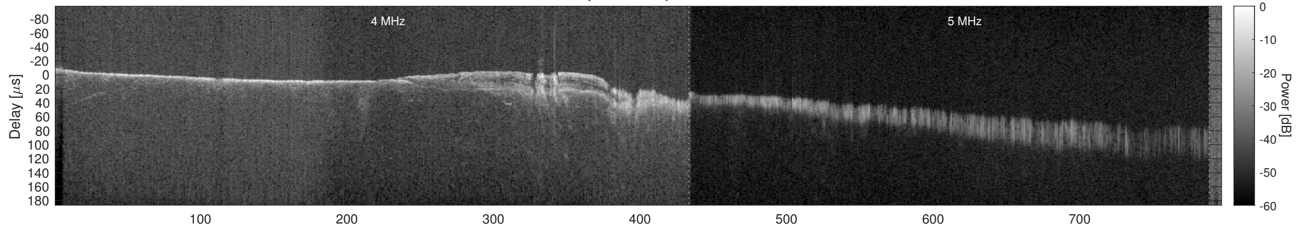
Orbit 9663, Window, Channel 1, Chapman
