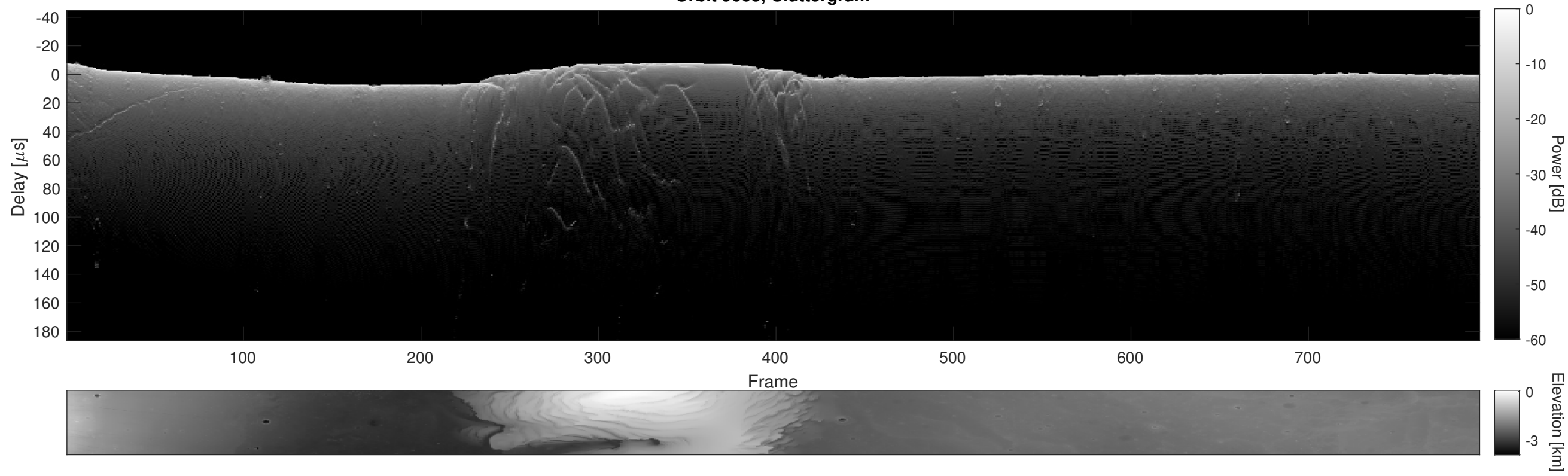
Orbit 9663, Cluttergram
