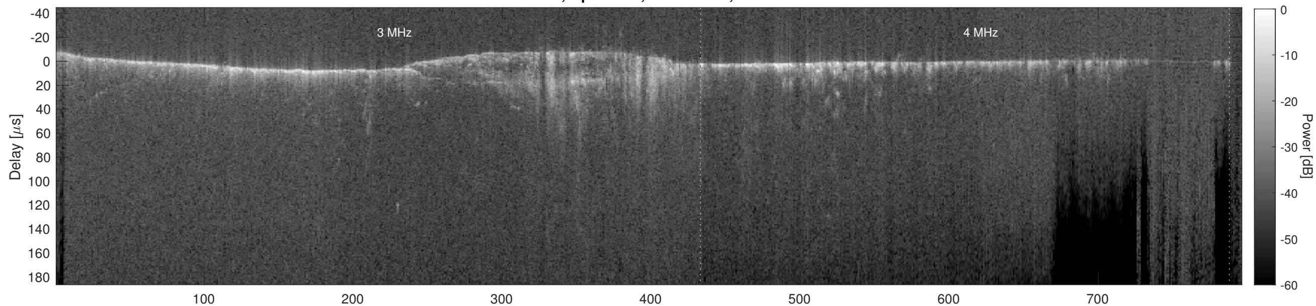
Orbit 9663, Cluttergram
