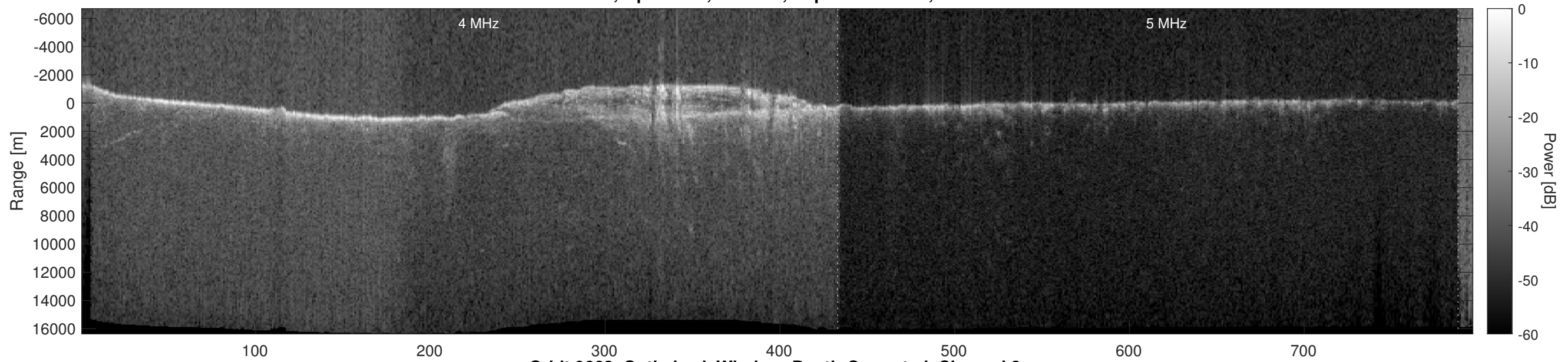
Orbit 9663, Optimized, Window, Depth-Corrected, Channel 2
