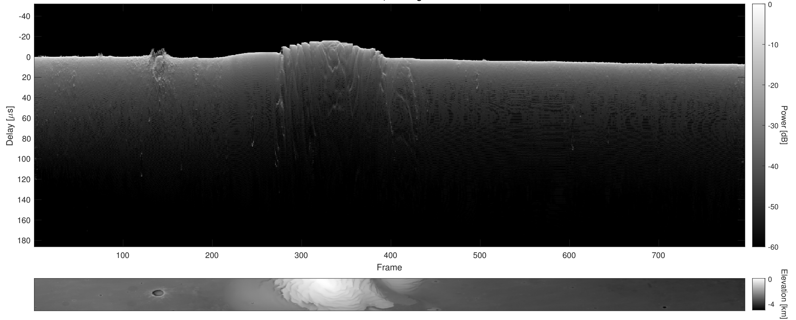
Orbit 9664, Cluttergram
