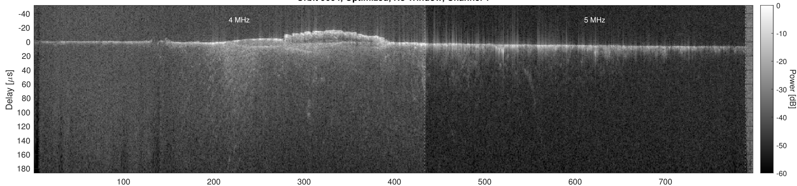
Orbit 9664, Optimized, No Window, Channel 2
