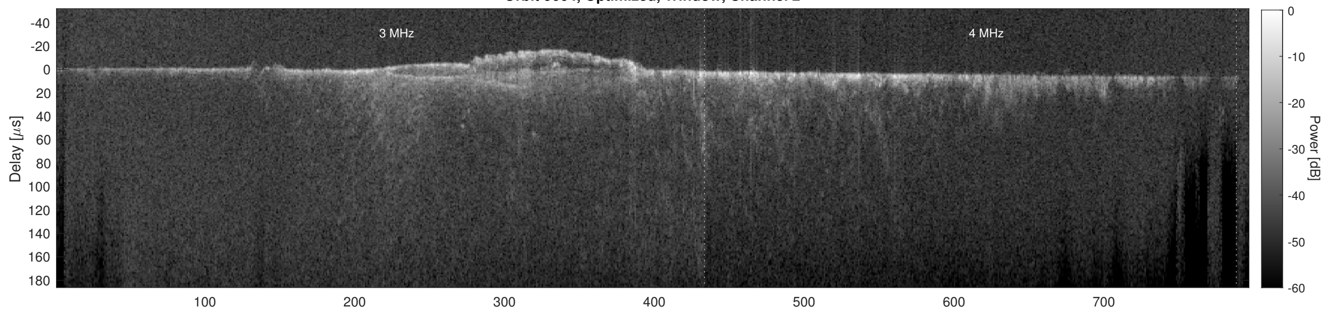
Orbit 9664, Cluttergram
