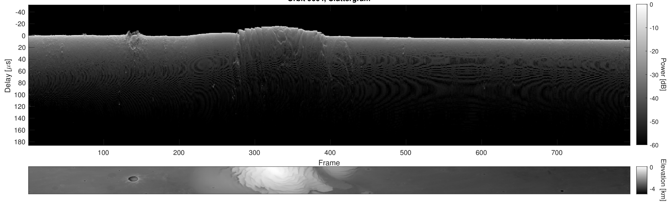
Orbit 9664, Cluttergram
