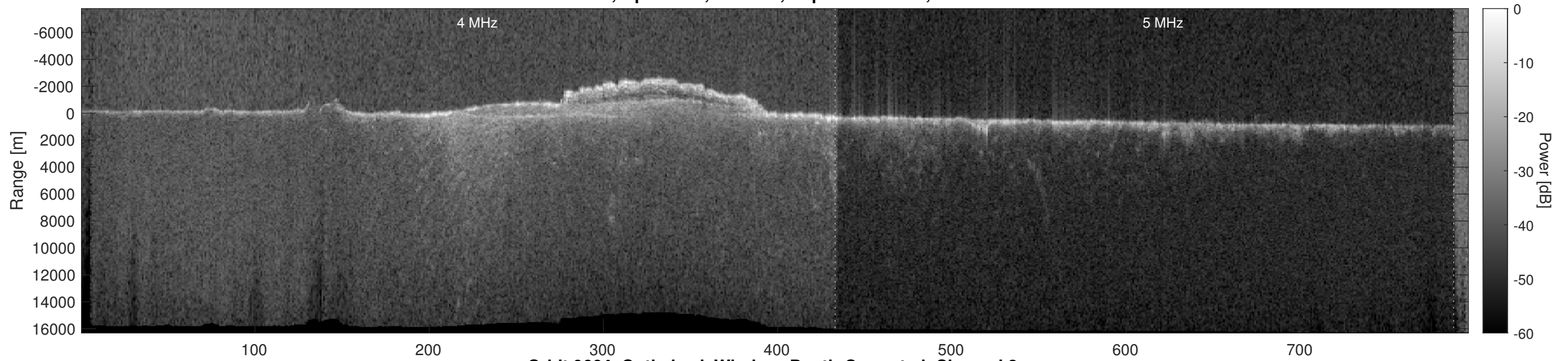
Orbit 9664, Optimized, Window, Depth-Corrected, Channel 2
