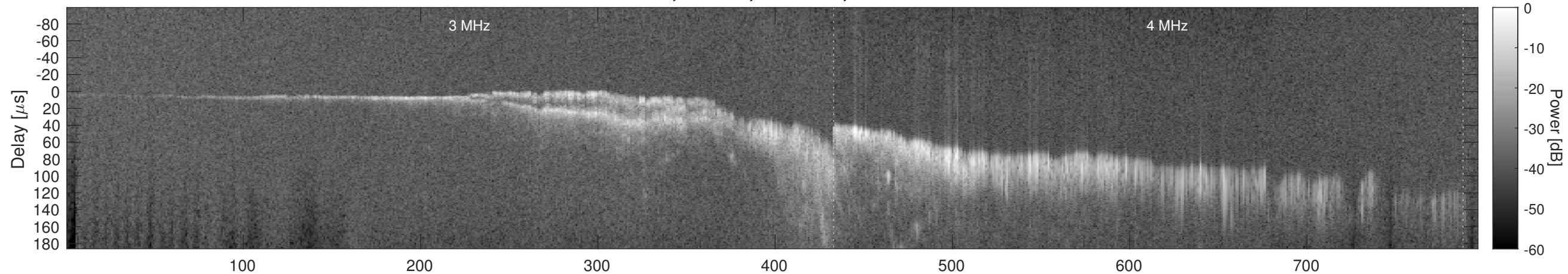
Orbit 9665, Window, Channel 2, Chapman
