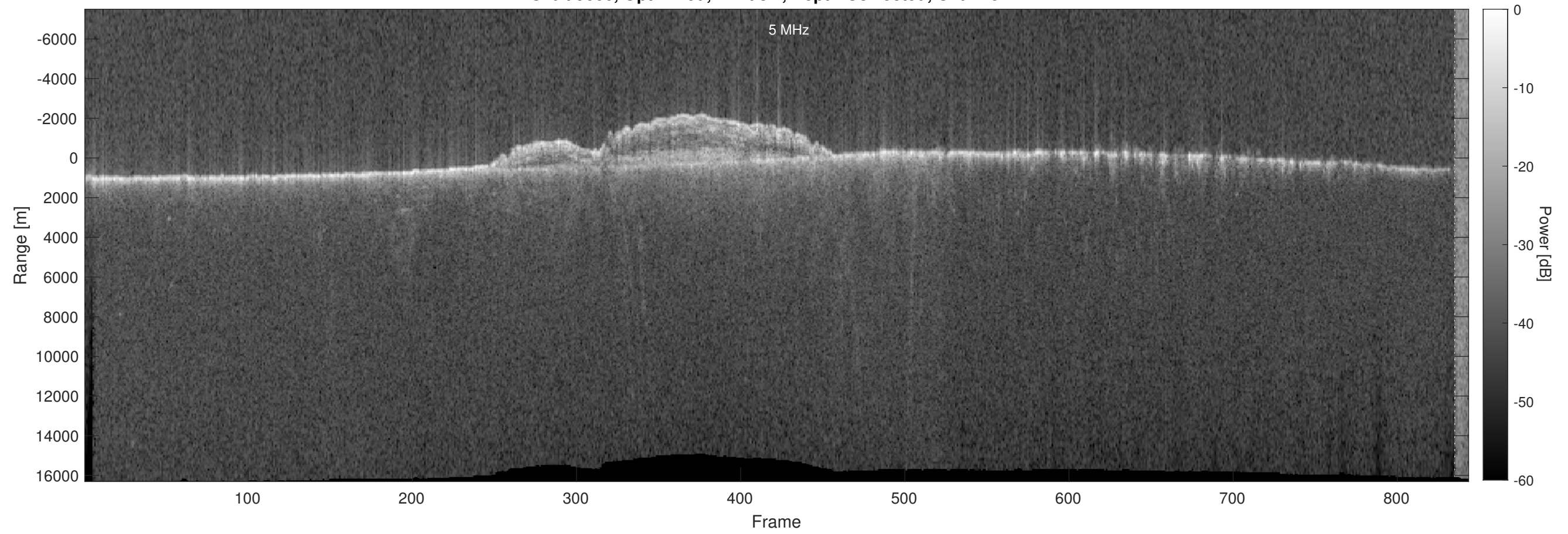
Orbit 9666, Optimized, Window, Depth-Corrected, Channel 2
