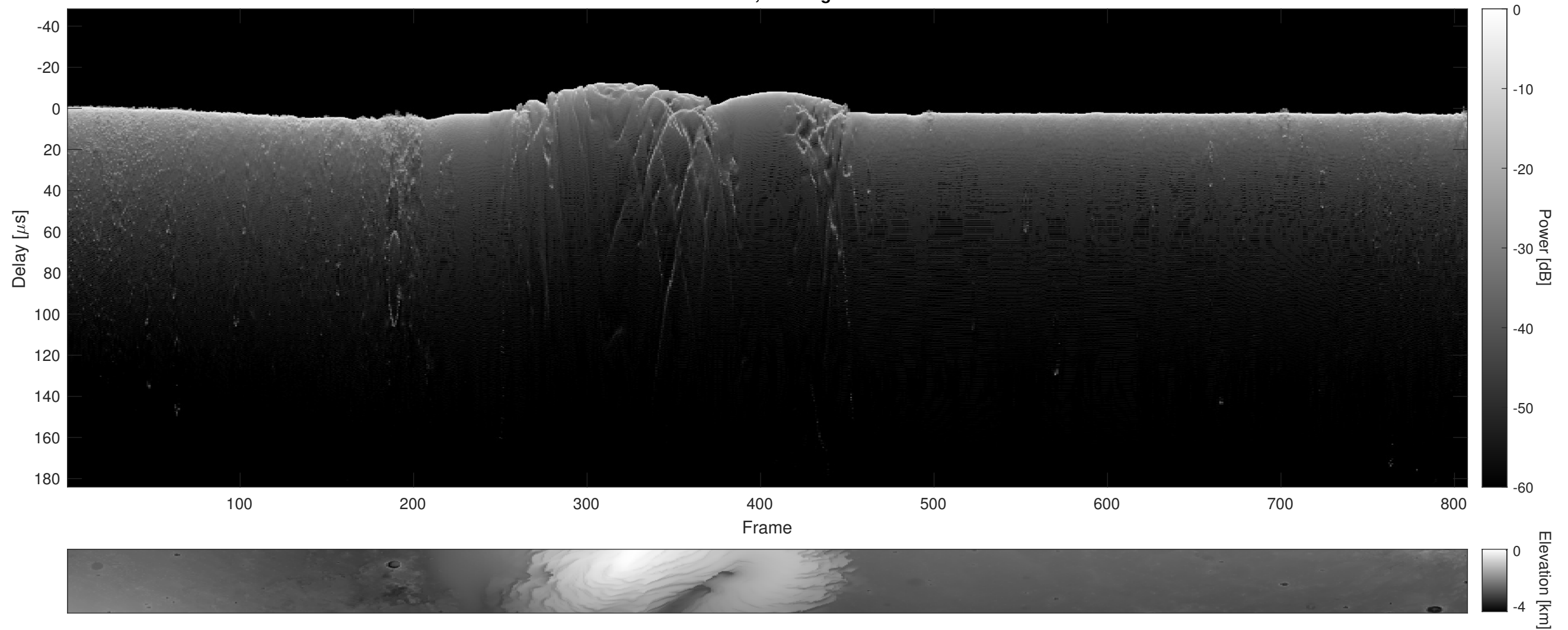
Orbit 9667, Cluttergram
