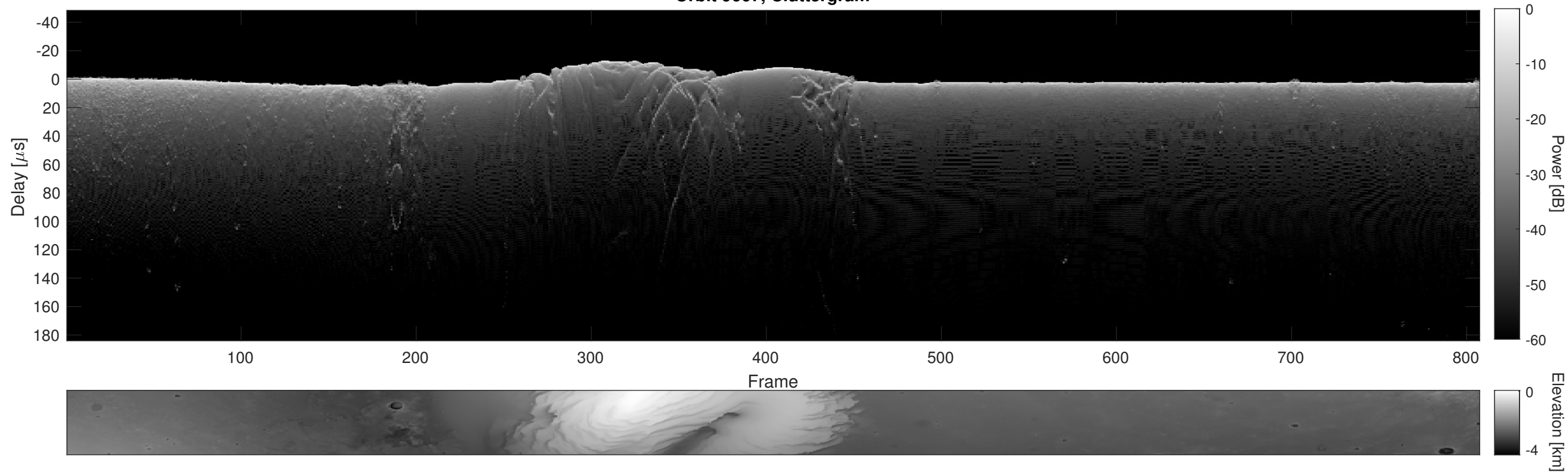
Orbit 9667, Cluttergram
