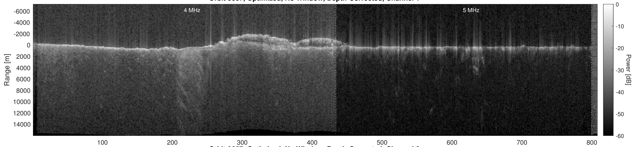
Orbit 9667, Optimized, No Window, Depth-Corrected, Channel 2
