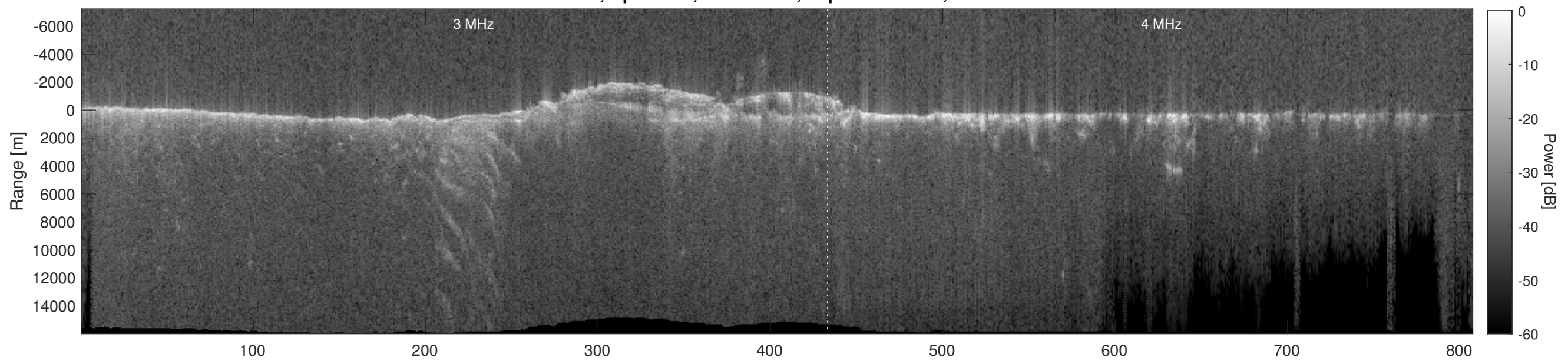
Orbit 9667, Depth-Corrected Cluttergram
