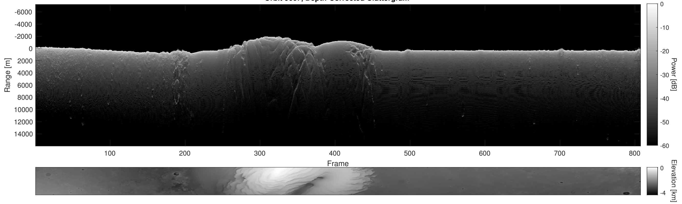
Orbit 9667, Depth-Corrected Cluttergram
