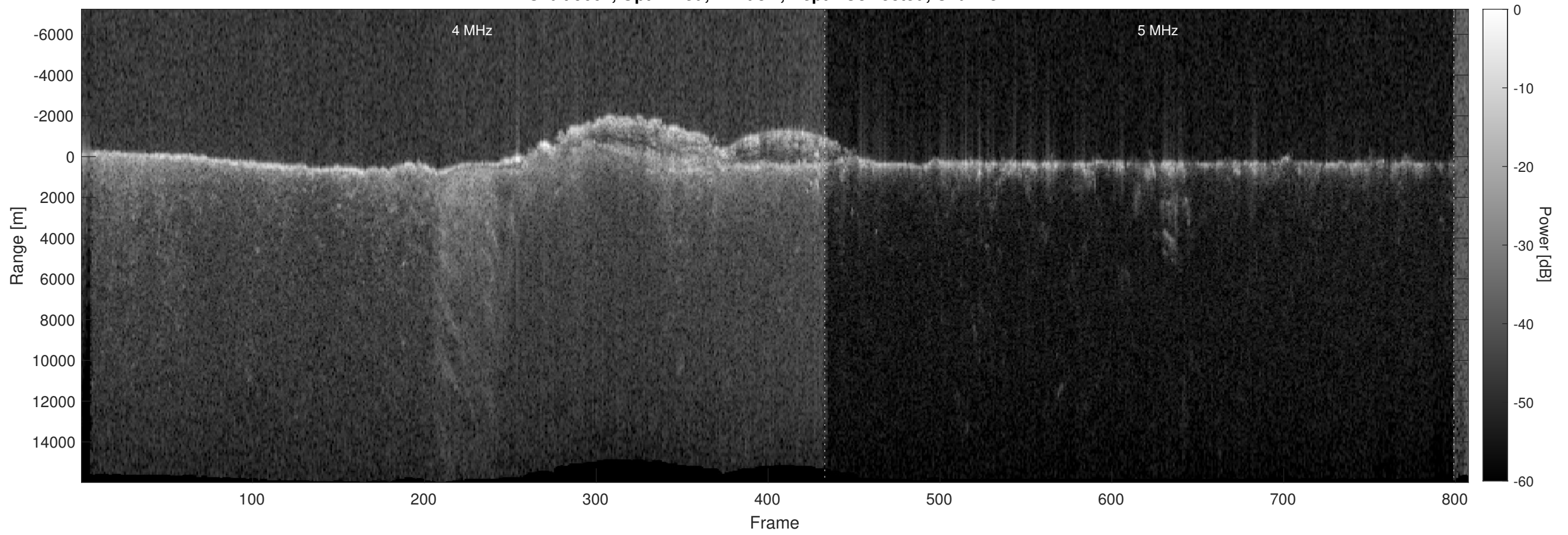
Orbit 9667, Optimized, Window, Depth-Corrected, Channel 2
